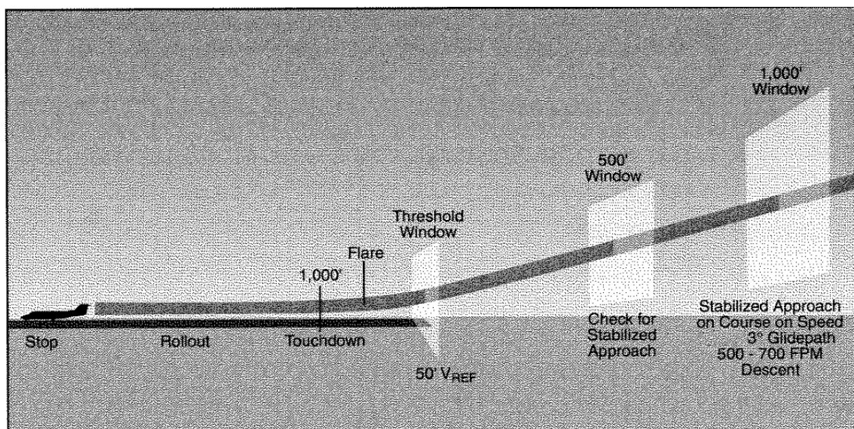
FIGURE 1-1. STABILIZED APPROACH
