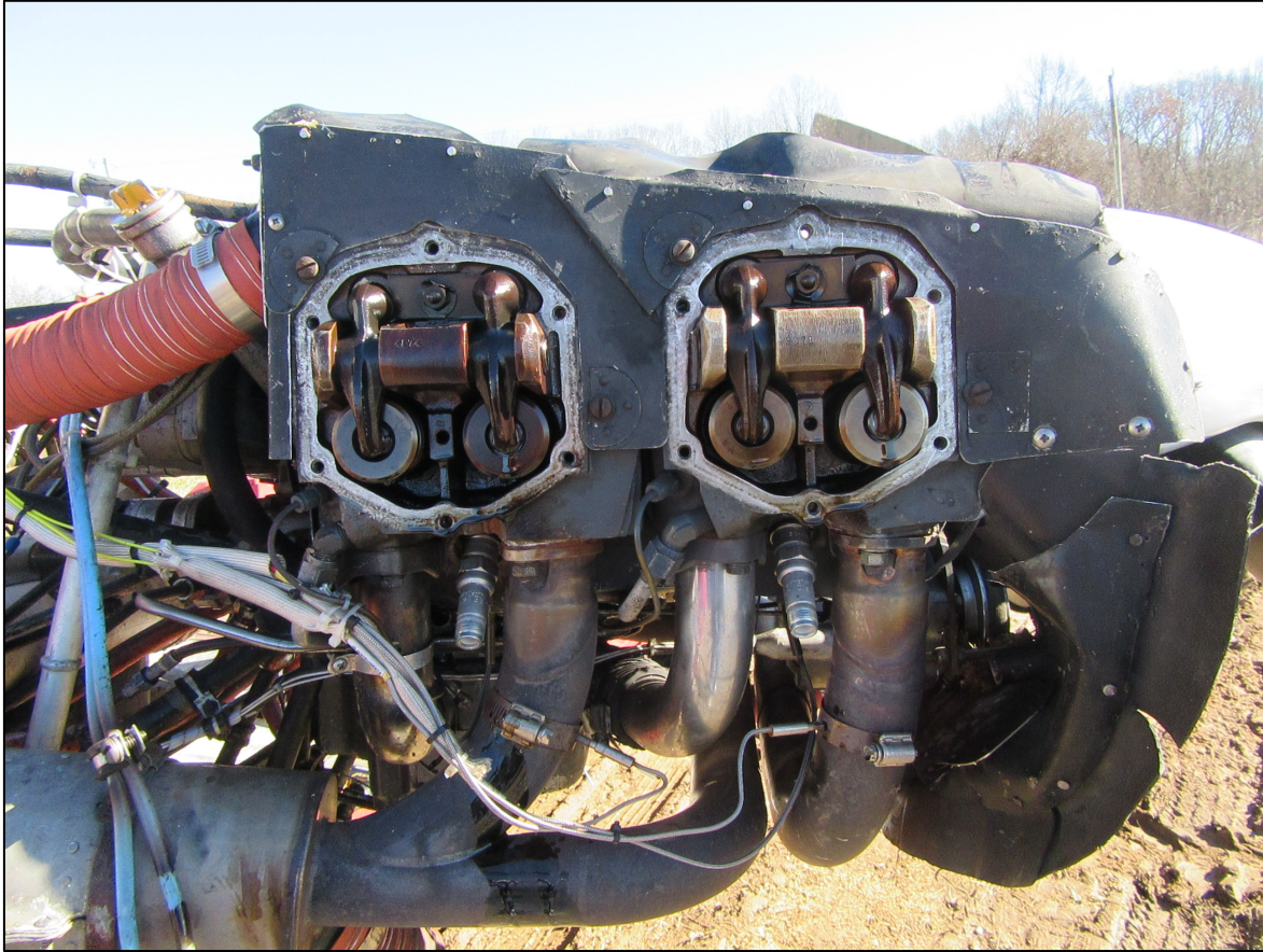
Photo 6 – View of the engine cylinders during engine examination. (Photo Courtesy of FAA)
