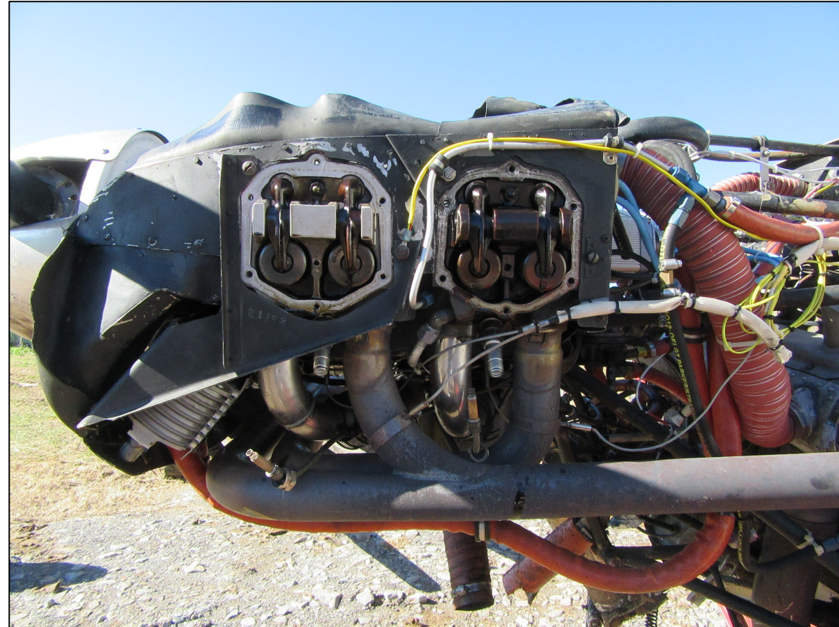
Photo 7 – View of the engine cylinders during engine examination. (Photo Courtesy of FAA)
