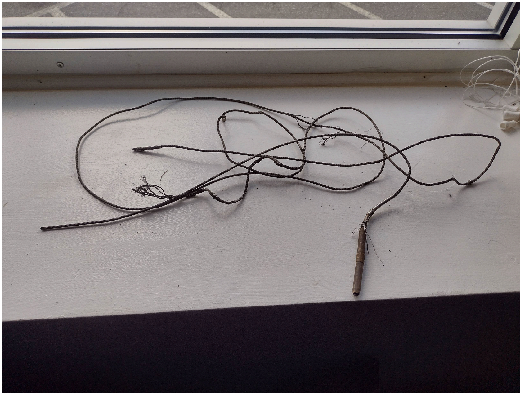
Photo 9 - Digital Photograph From AMF Aviation. Loose Elevator Control Cable retained For NTSB Examination. Note the Fractured Turnbuckle Eye.
