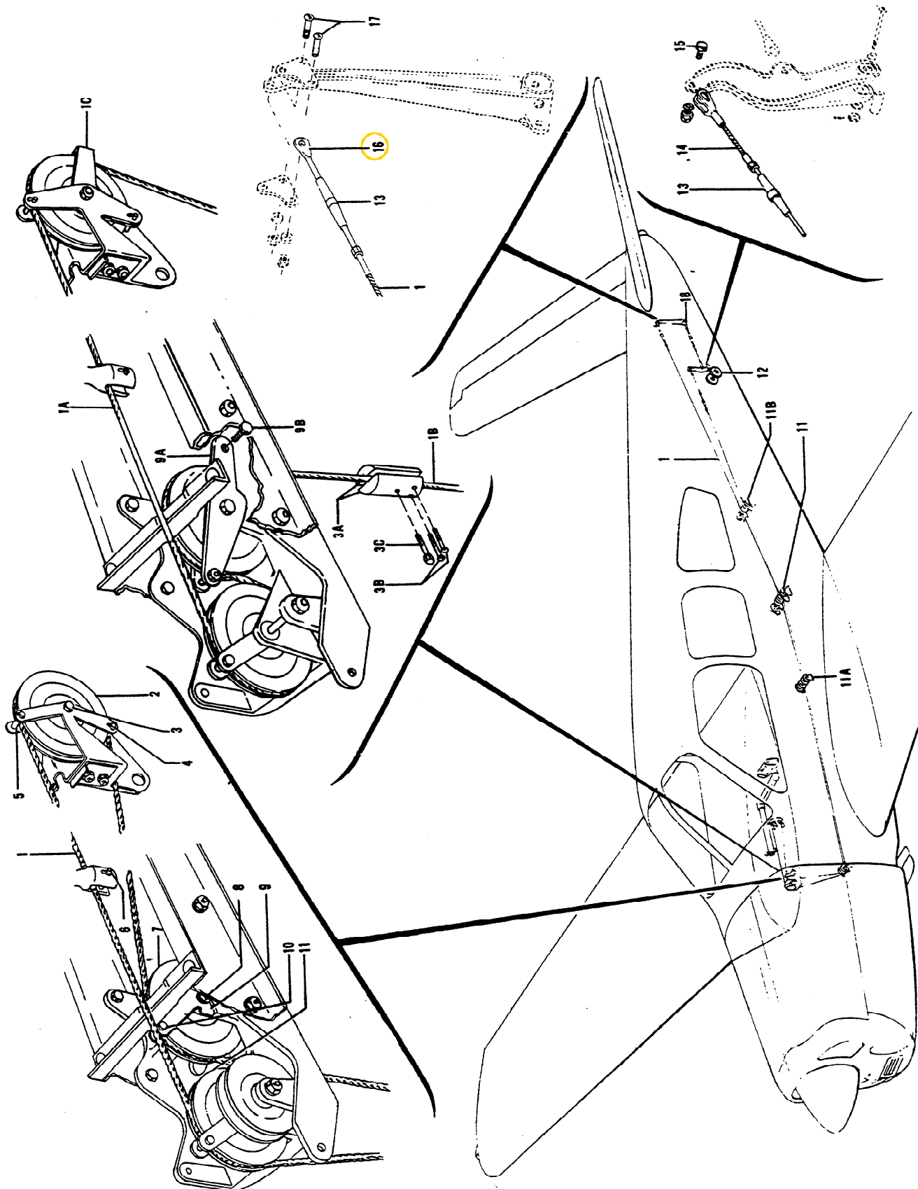
Figure 28. Elevator Control System
