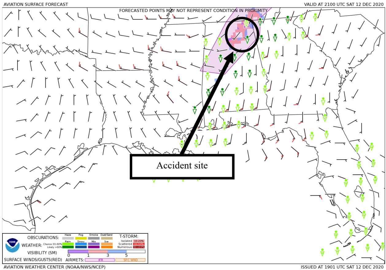
Figure 2 – GFA Surface Forecast valid at 1500 CST with forecast issued at 1301 CST.
