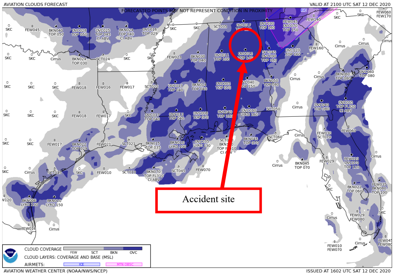
Figure 3 – GFA Aviation Clouds Forecast valid at 1500 CST with forecast issued at 1002 CST.
