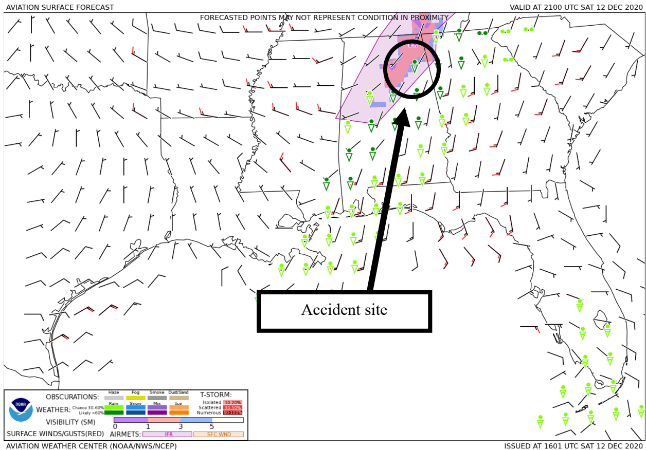
Figure 1 – GFA Surface Forecast valid at 1500 CST with forecast issued at 1001 CST.
