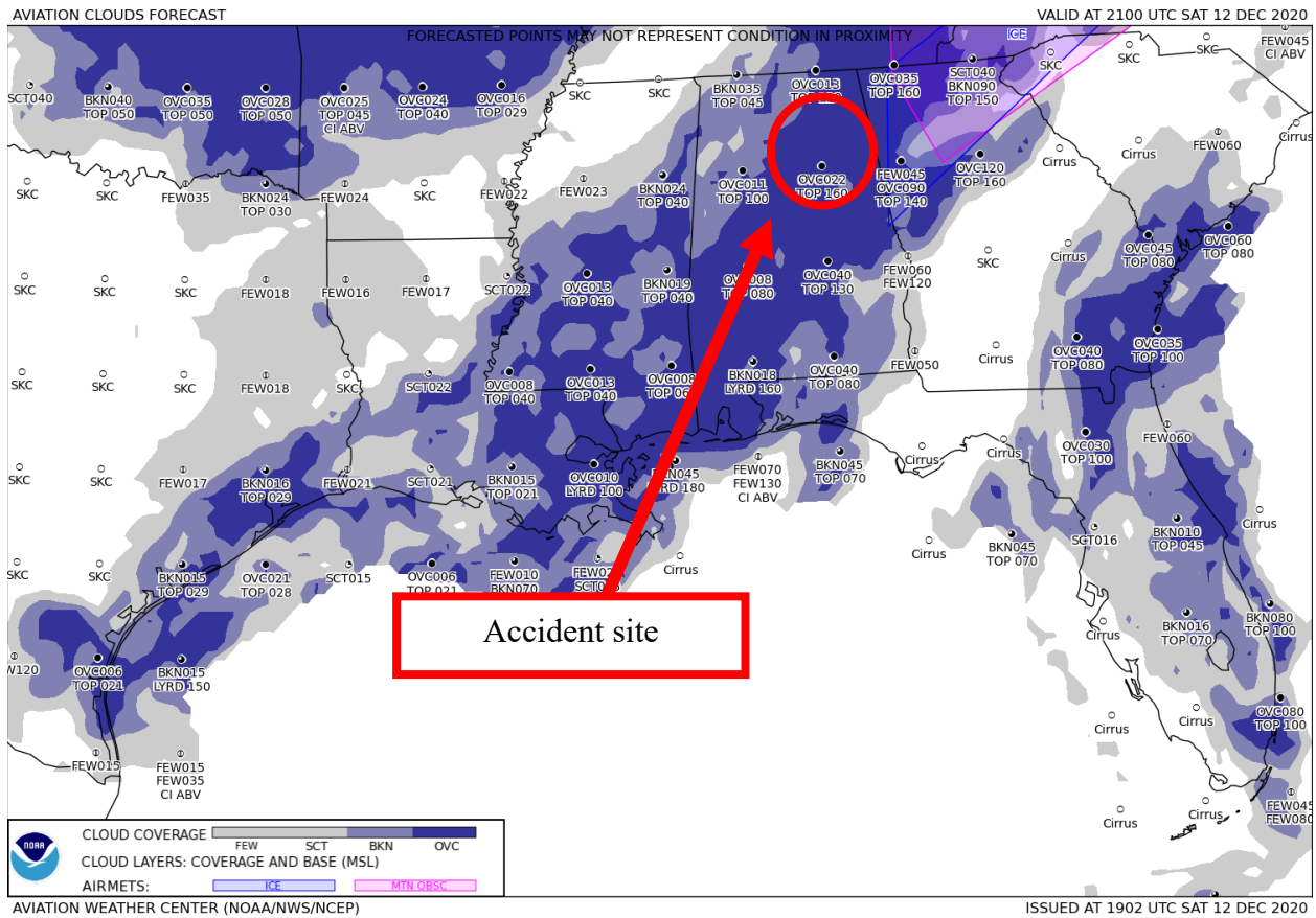
Figure 4 – GFA Aviation Clouds Forecast valid at 1500 CST with forecast issued at 1302 CST.
