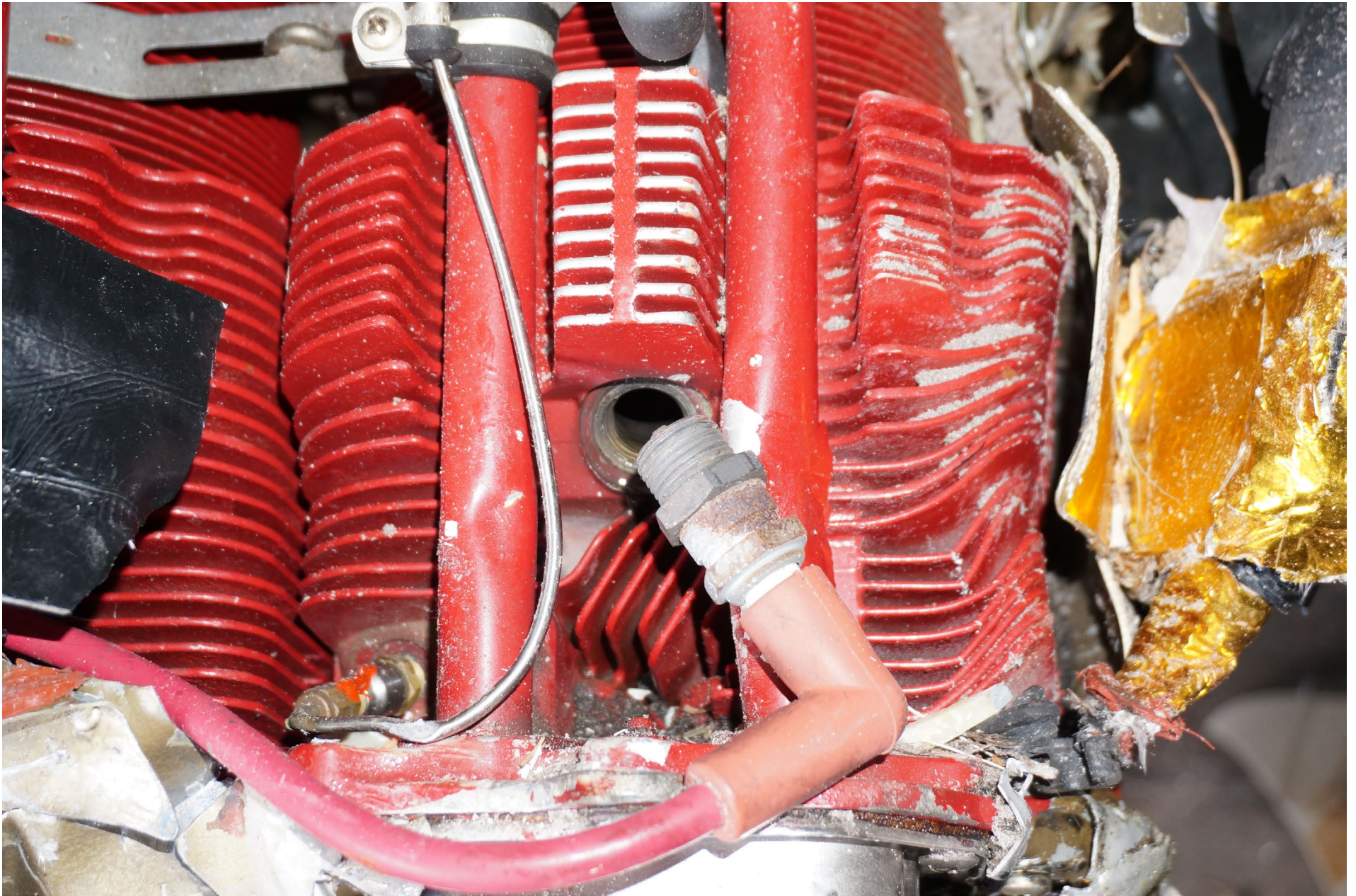
Photo 9 – No. 1 Top Spark Plug and Adaptor
