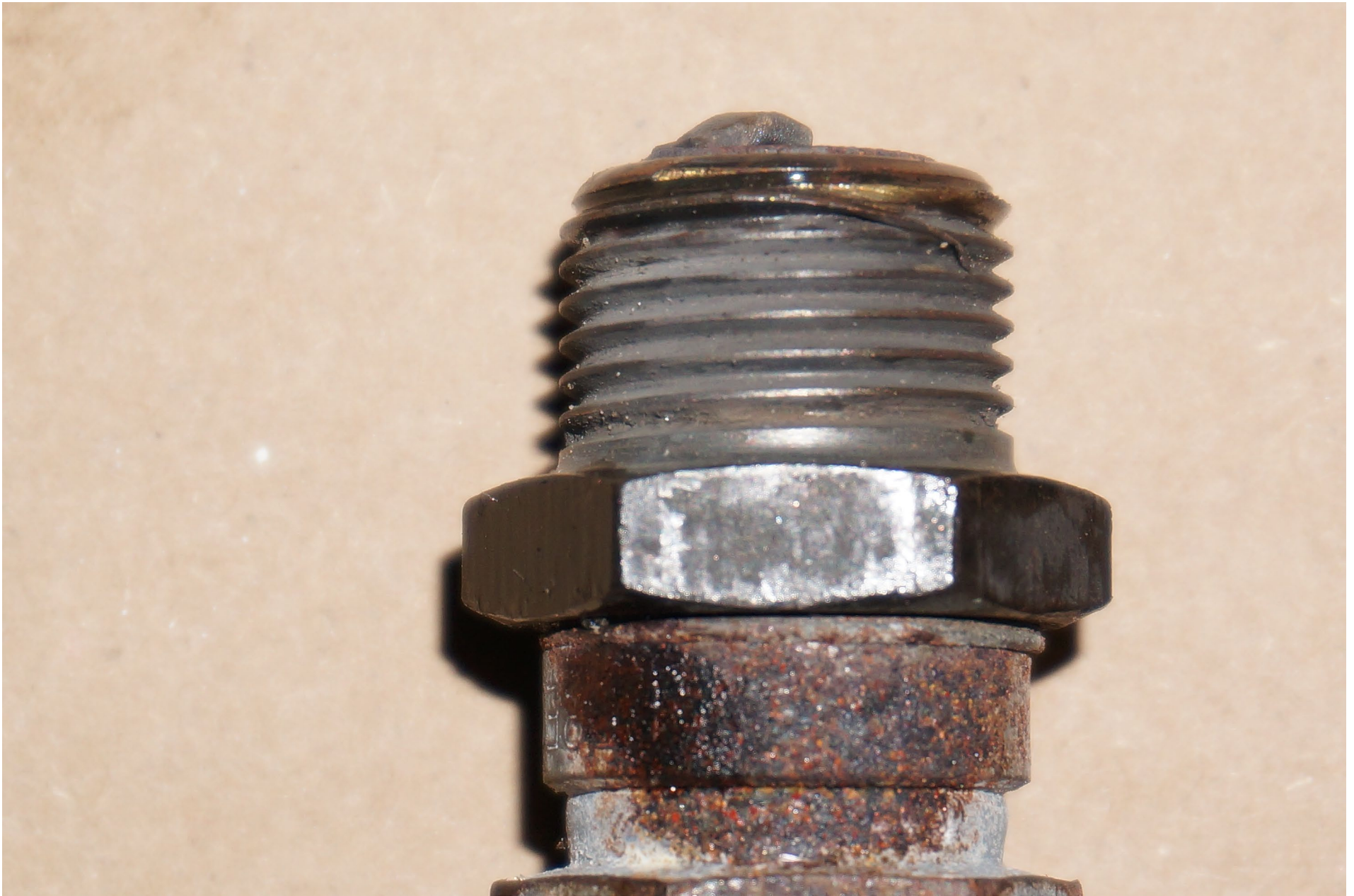
Photo 11 – Close Up of Damaged Threads on Adaptor
