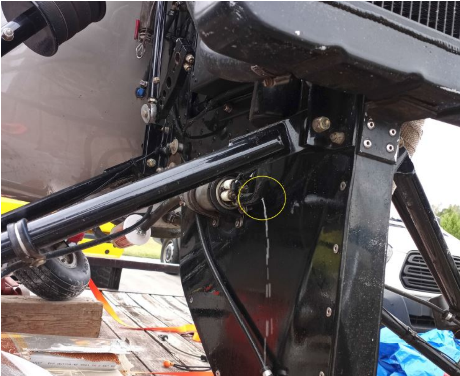
Photo 3 – View of fuel actively leaking postaccident from a rubber fuel line (Photo Courtesy of FAA)
