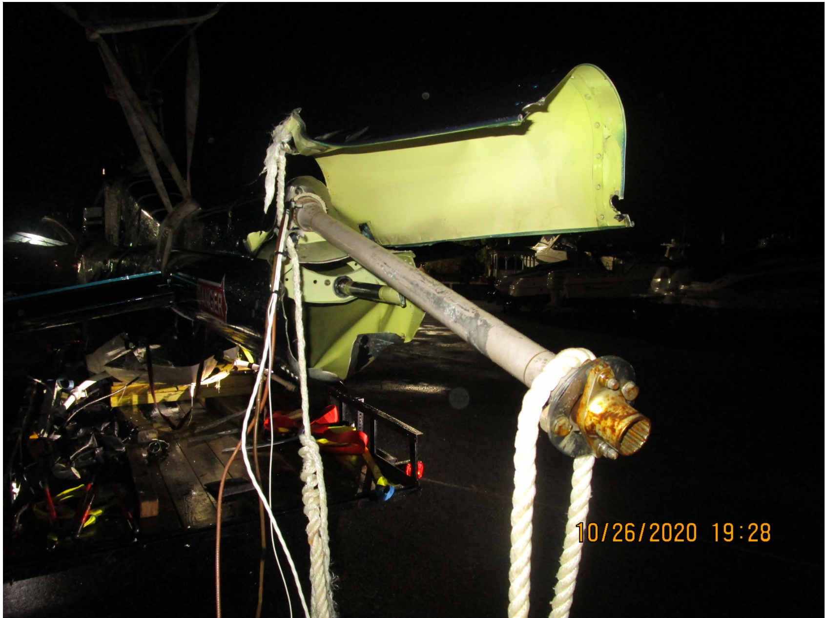
Photo 5 - Digital Photograph From Federal Aviation Administration. View of the Tail Rotor Drive Shaft and Fractured Tail Rotor Control Fixed Tube Assembly.
