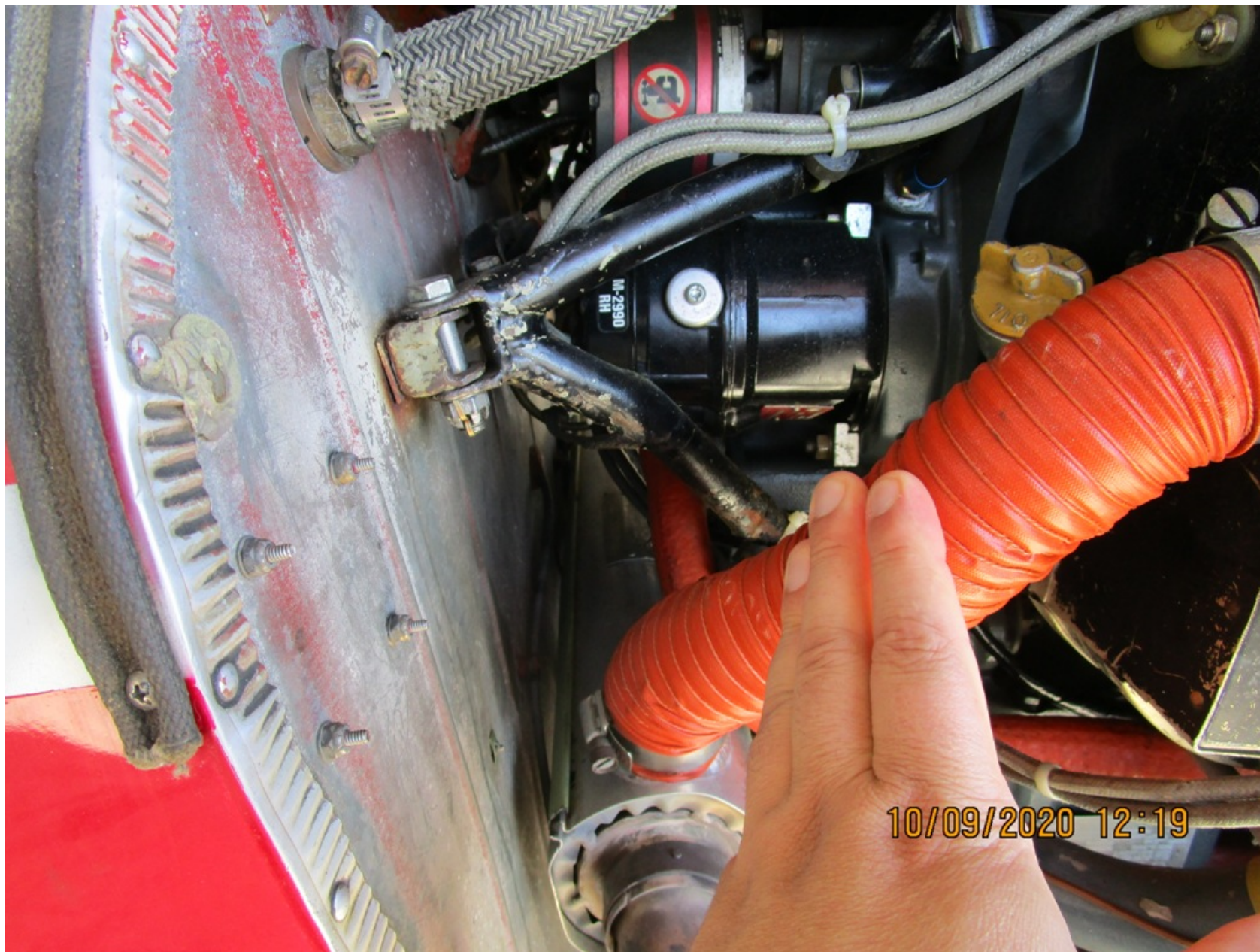
Photo 4 - Digital Photograph Provided by FAA. Right Side View of the Engine Compartment Following Recovery. Note the Damage to the Engine Mount.
