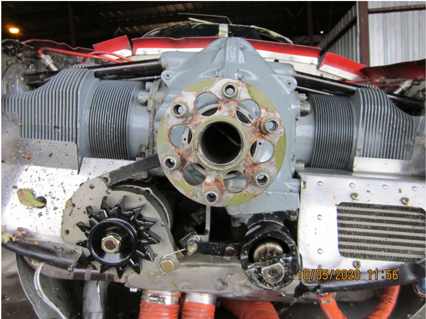
Photo 3 - View of Crankshaft with Crankshaft Plug Missing (courtesy FAA)
