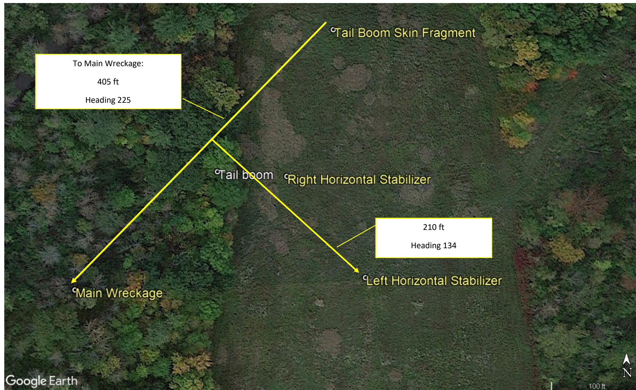
Figure 1 Wreckage Diagram
