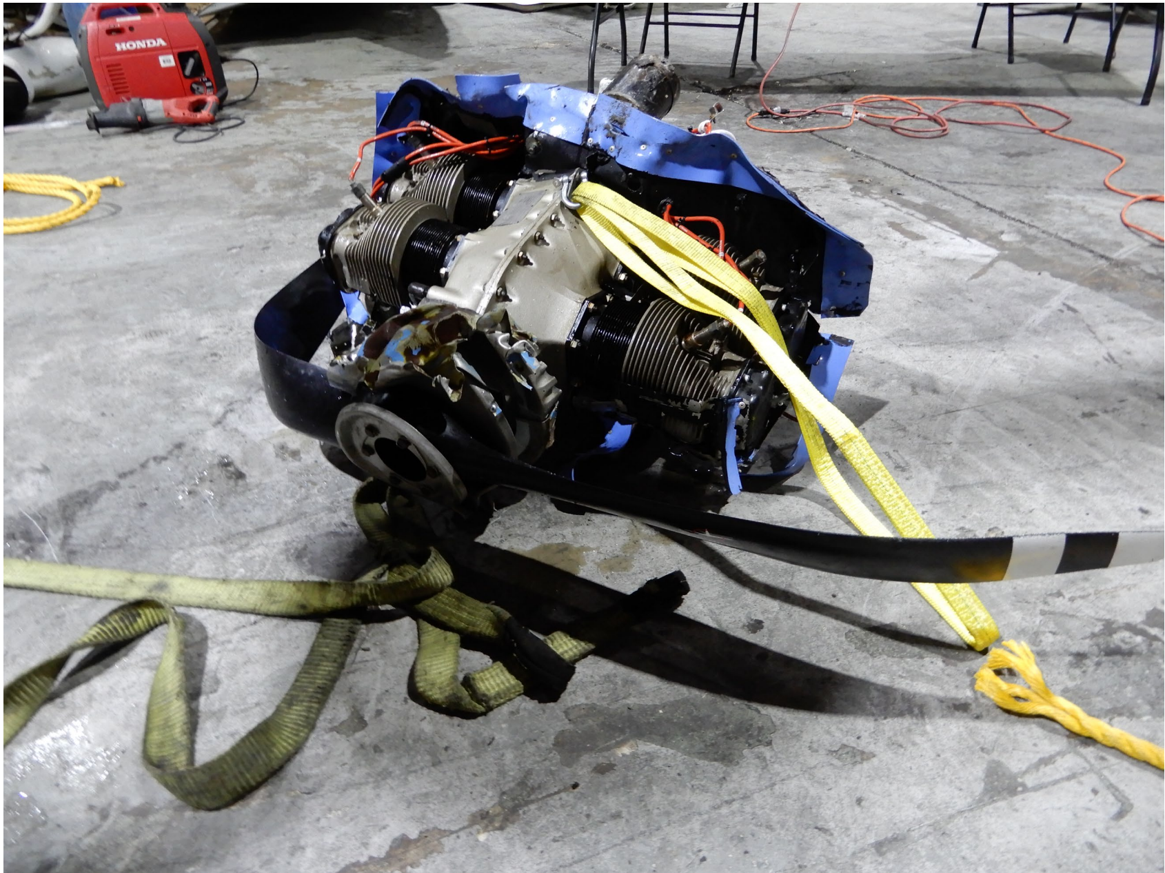
Photo 9 – Engine and Propeller (NTSB Photo)
