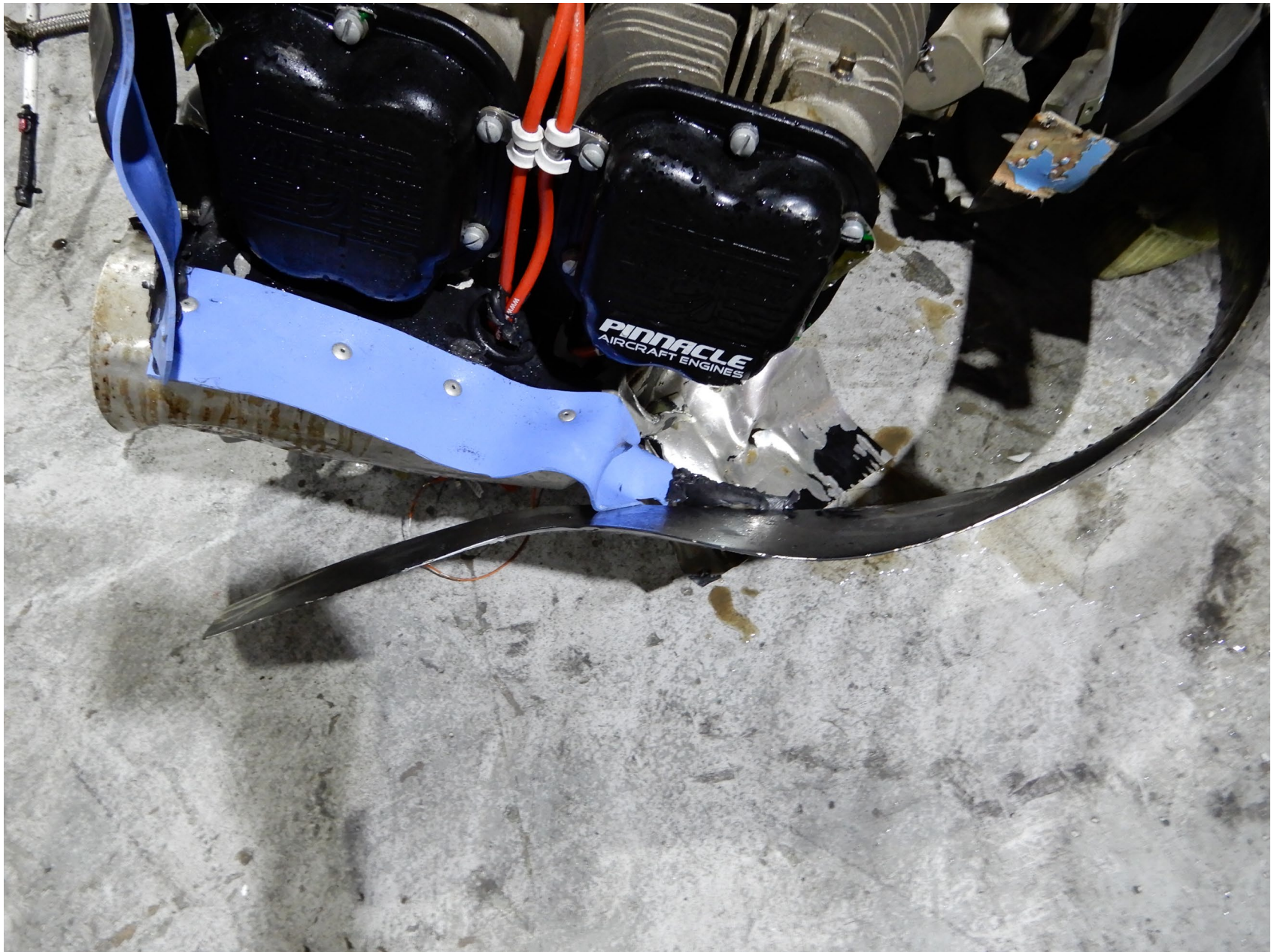
Photo 10 – Propeller Blade (NTSB Photo)
