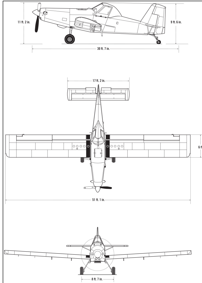
Drawing of accident airplane model (Source: Airplane Flight Manual)
