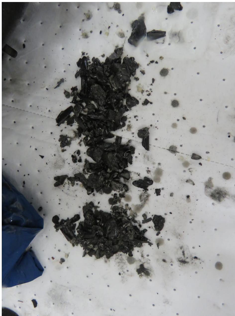
Photo 17 – Metallic Debris from Oil Sump – Courtesy of Lycoming Engines
