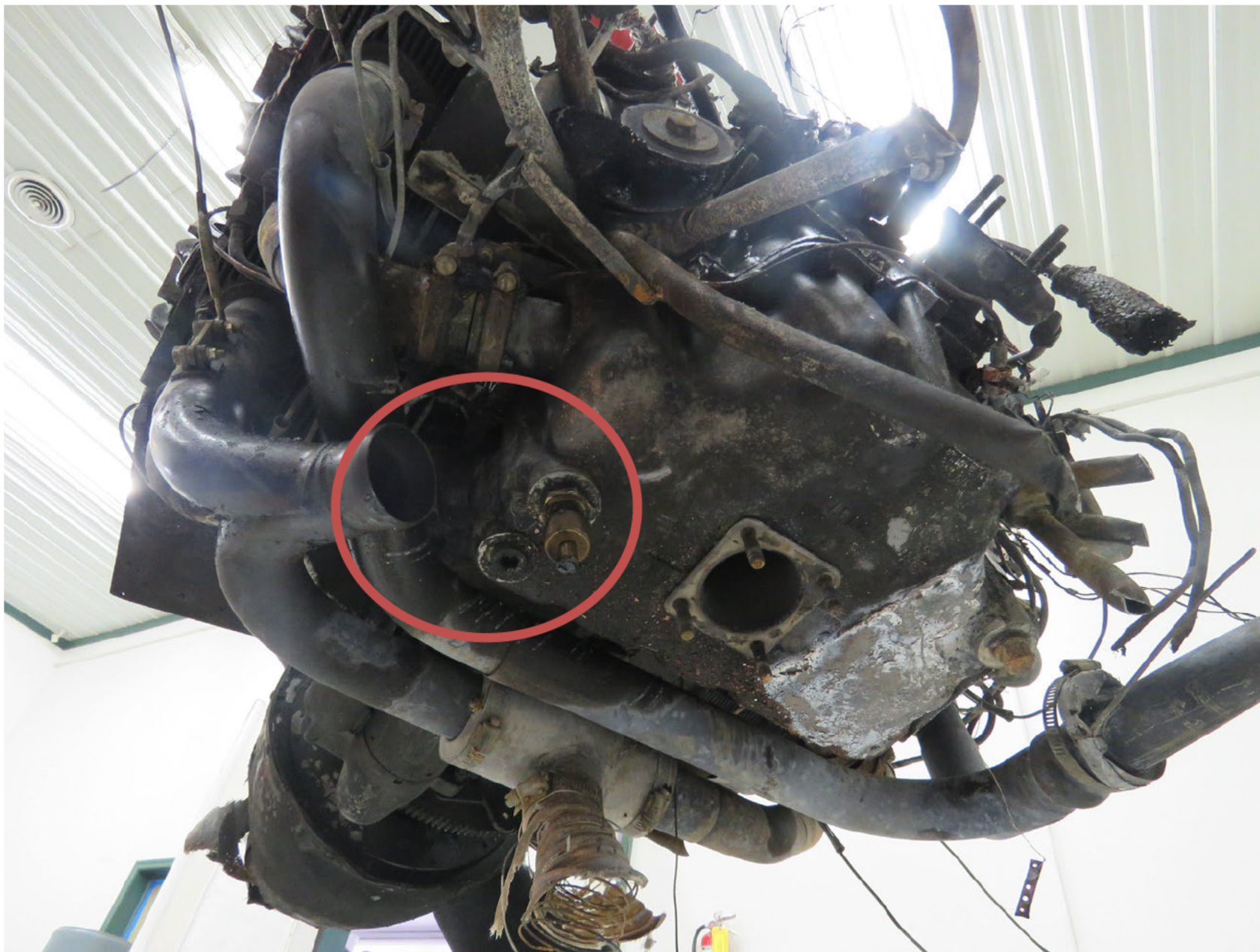
Photo 18 – Exhaust Stack and Oil Quick Drain – Courtesy of Lycoming Engines
