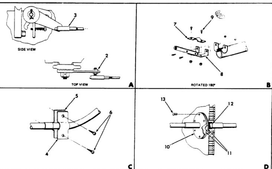
Throttle Control Installation Figure 73-1
