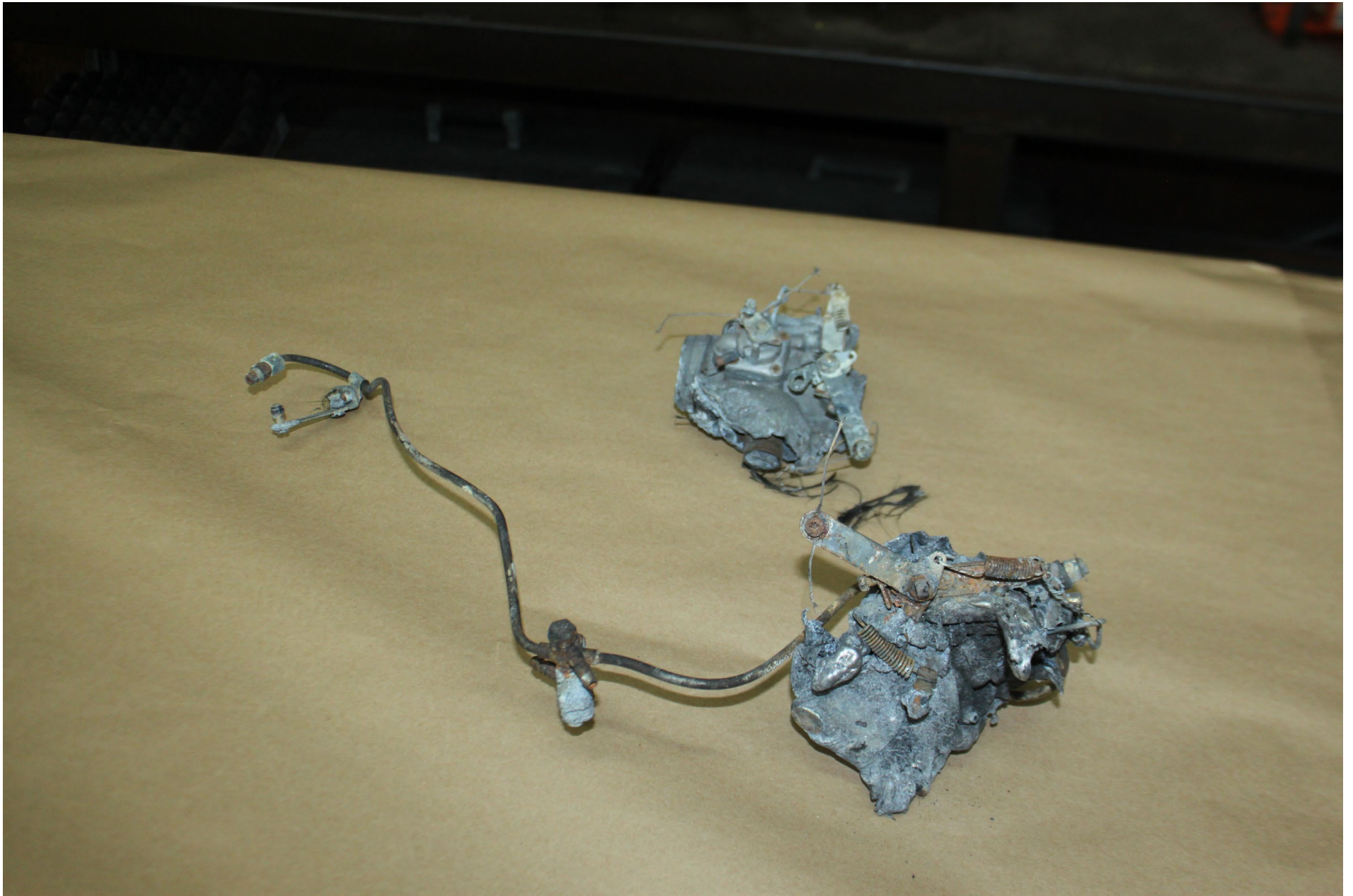
Photo 6 - NTSB Digital Photograph. View of the Extensively Heat Damaged Carburetors. Note the Nos. 1/3 Carburetor is in the Foreground and the Nos. 2/4 Carburetor is in the Background.
