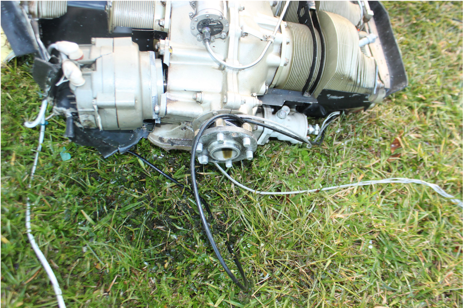
Photo 4 - NTSB Digital Photograph. View of Front Portion of the Engine. Note the Insulated Powerline Wrapped Around the Crankshaft and the Separated Propeller.
