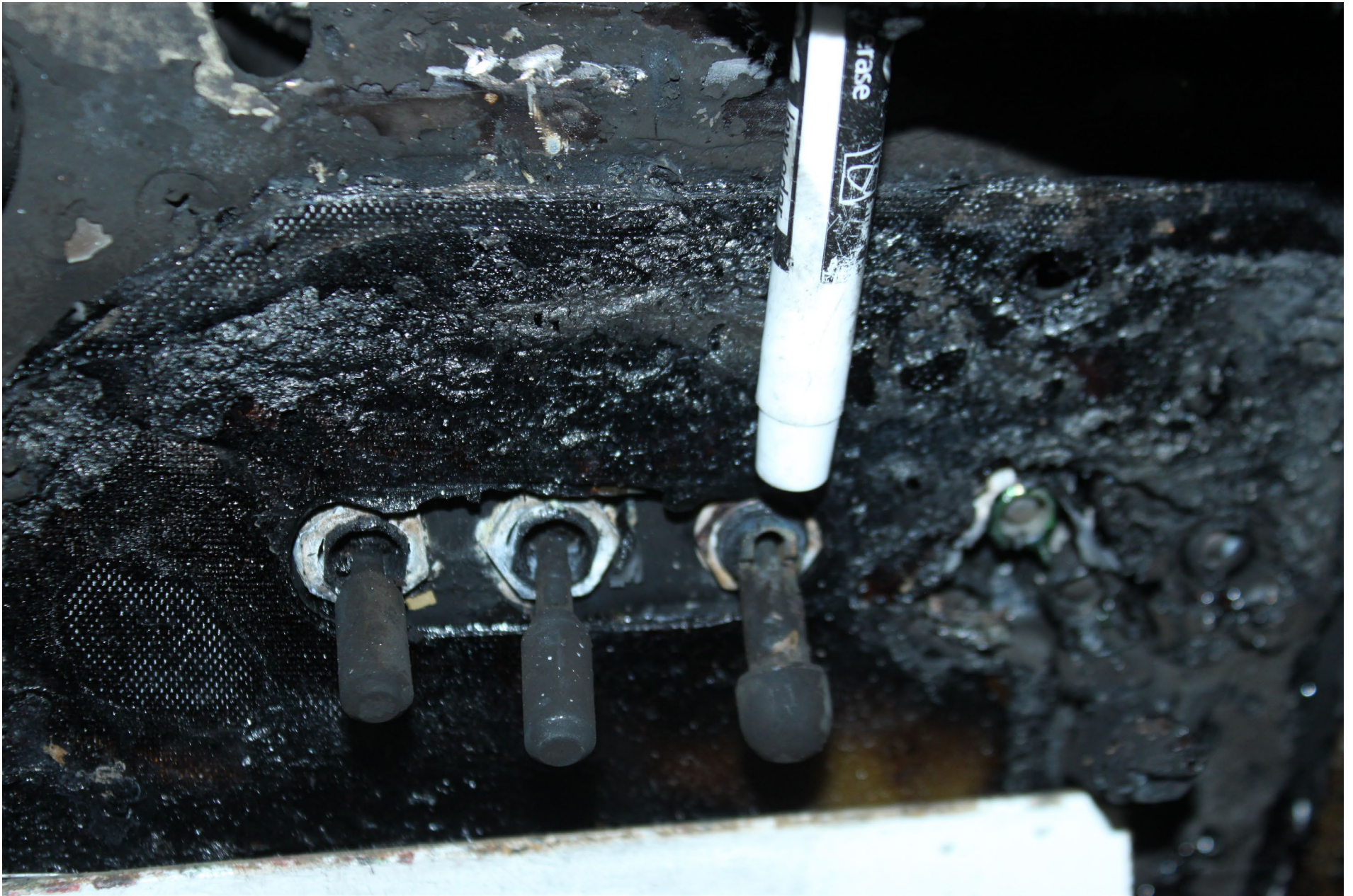
Photo 11 - NTSB Digital Photograph. Pen points to Auxiliary Fuel Pump Switch.
