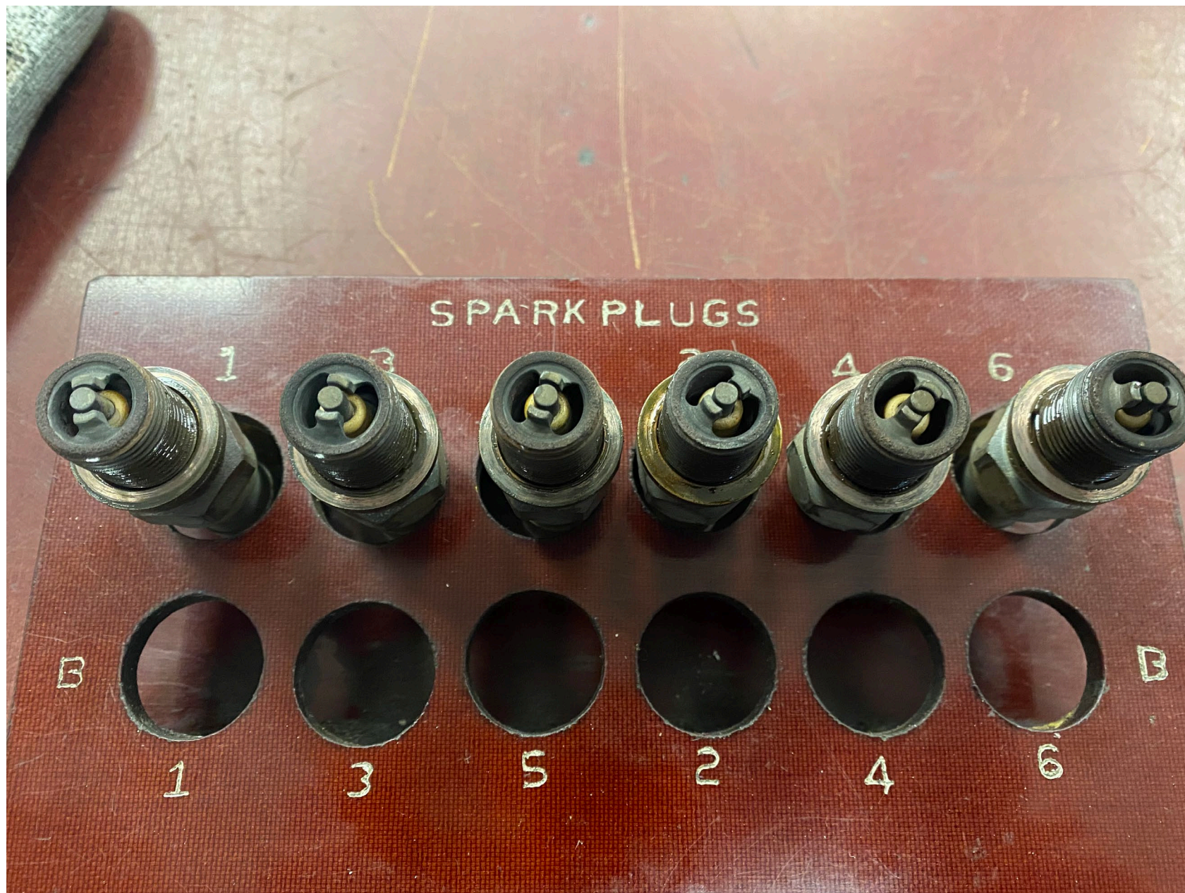
Photo 16 - Continental Aerospace Technologies Digital Photograph. View of the Cylinder Portions of All Top Spark Plugs Following the Last Full Power Engine Run. Note the Normal Color.
