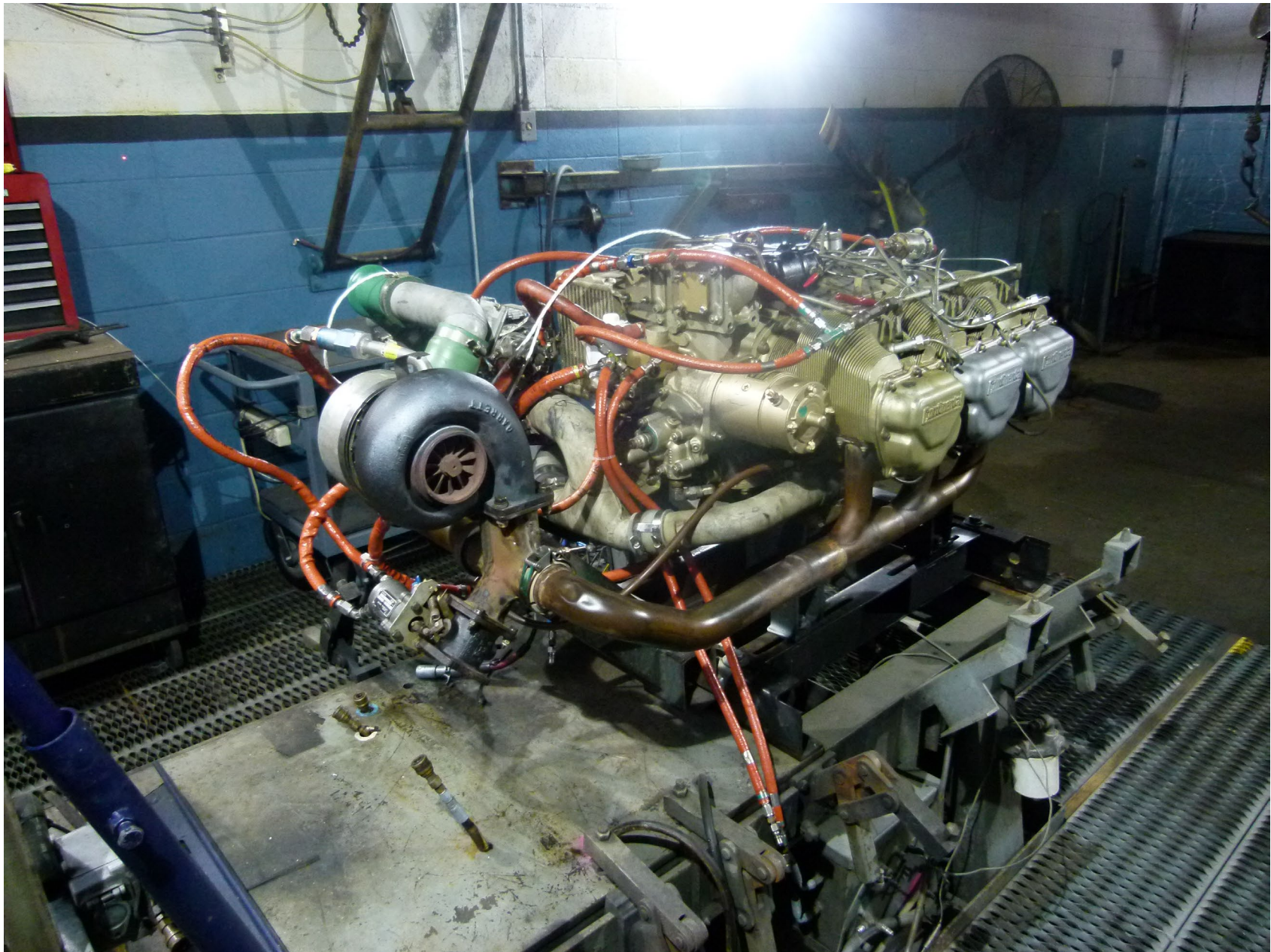
Photo 17 - Continental Aerospace Technologies Digital Photograph. Right Rear View of the Engine in the Test Cell Before Mounting Test Club Propeller.
