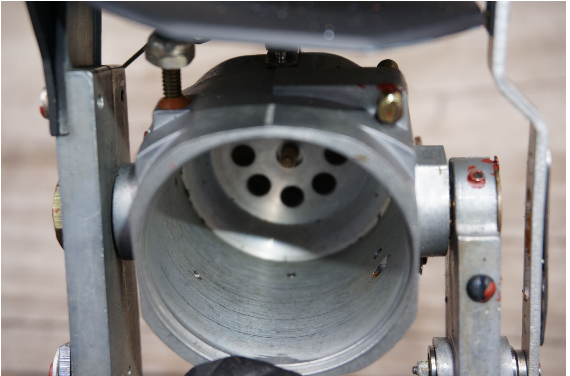
Photo 13 – Attitude Indicator Gyro Housing
