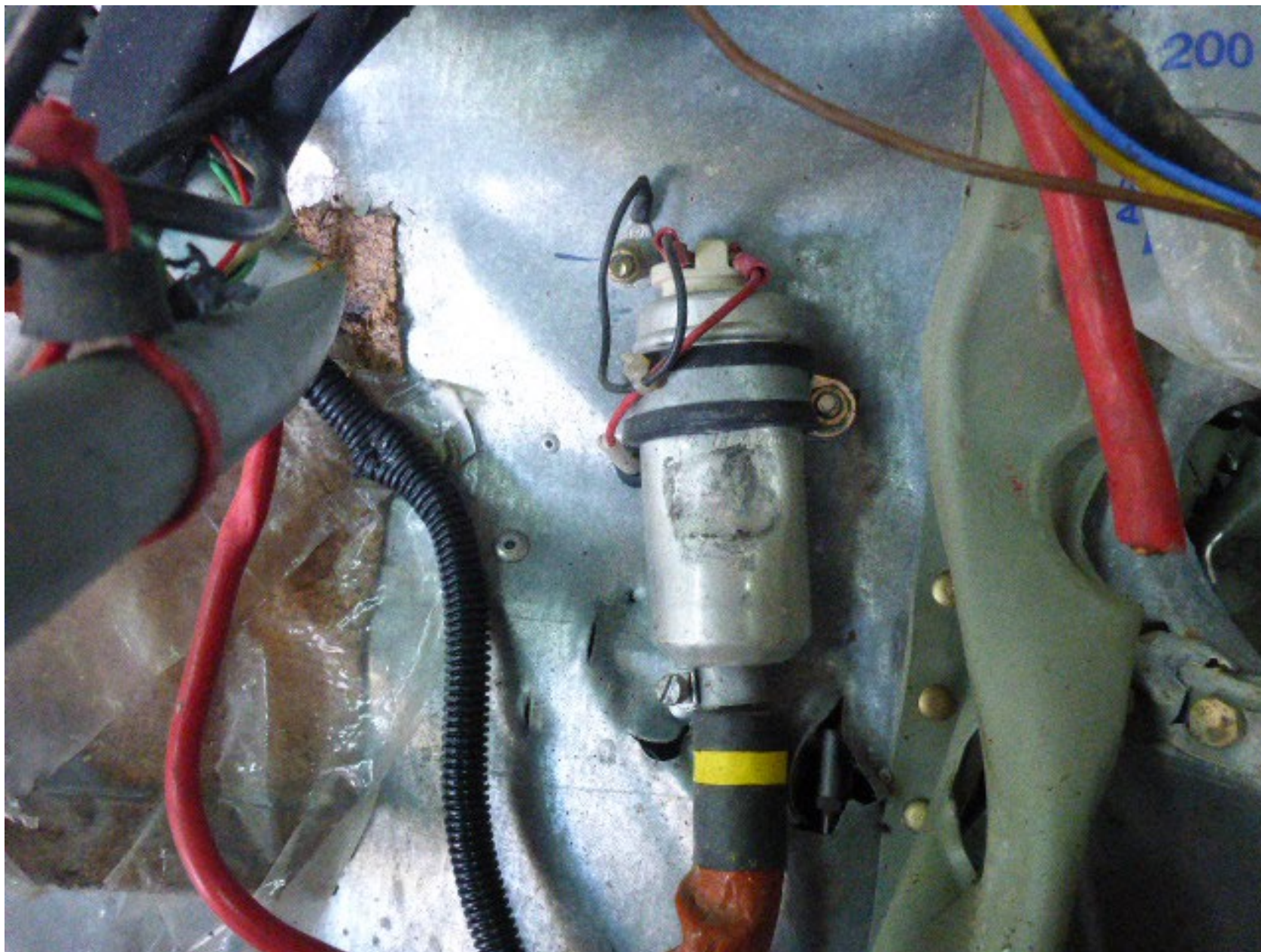
Photo 8 – Automotive installed fuel pump
