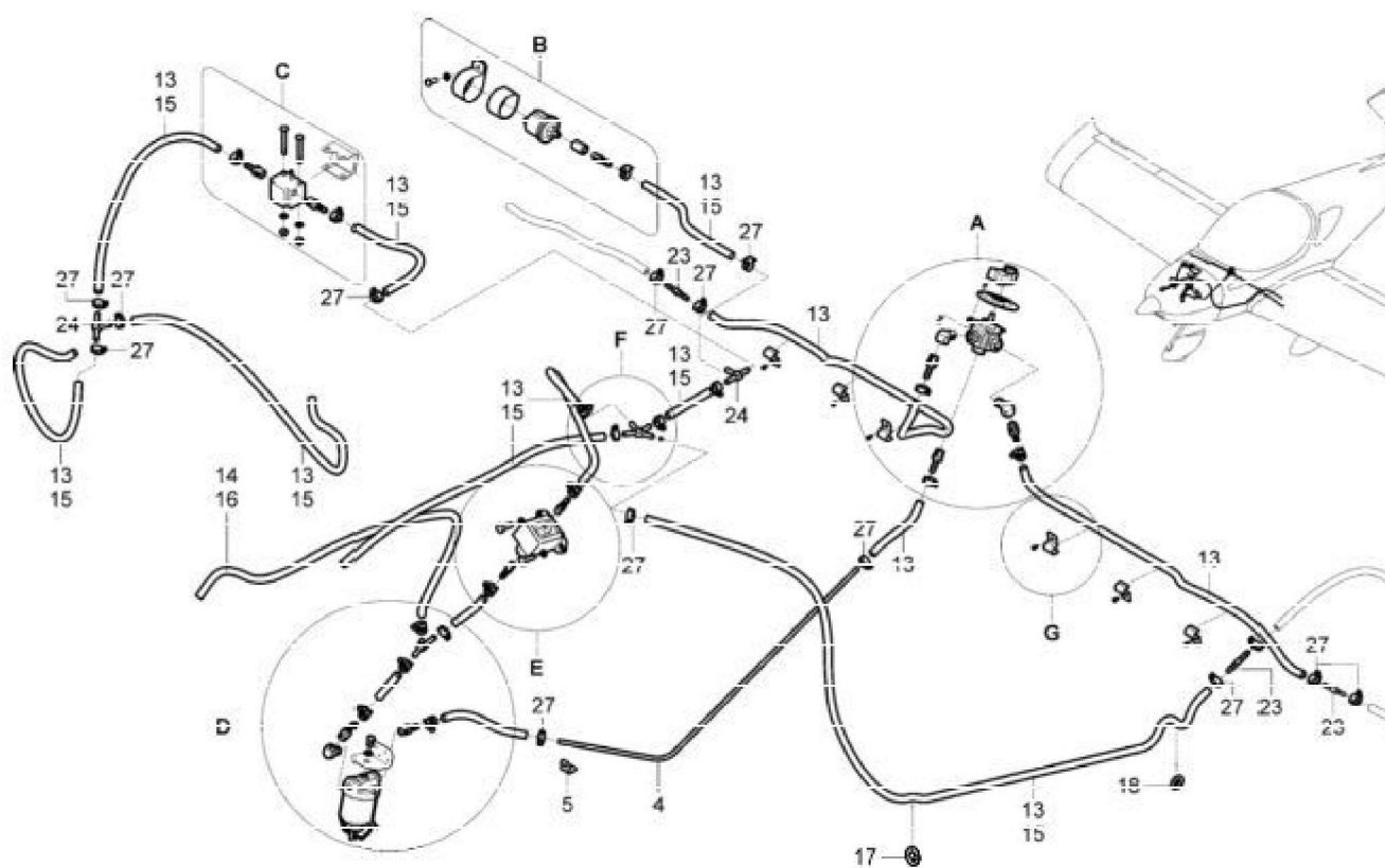
Figure 28-20-03, Fuel System
