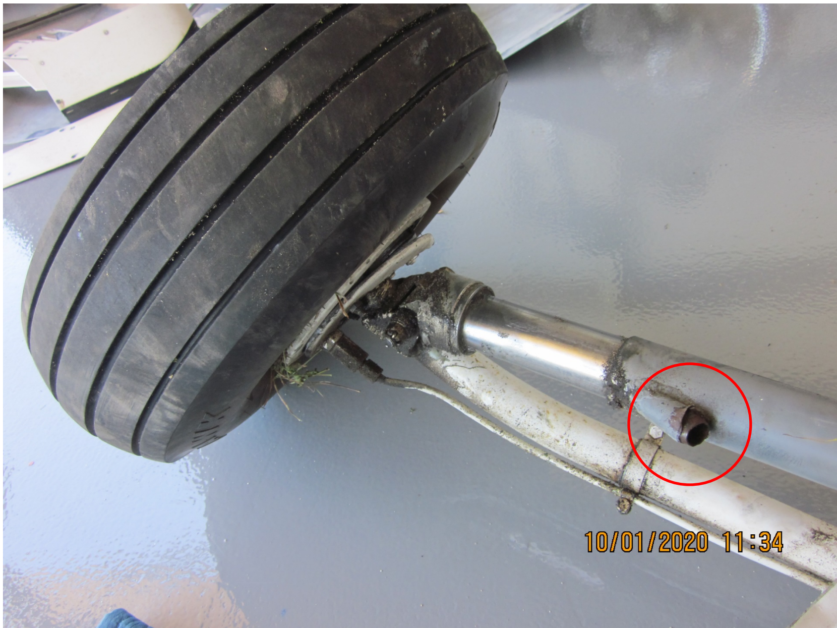
Figure 1 – View of the corrosion visible on the left landing gear airframe cross tube (Photo Courtesy of FAA)
