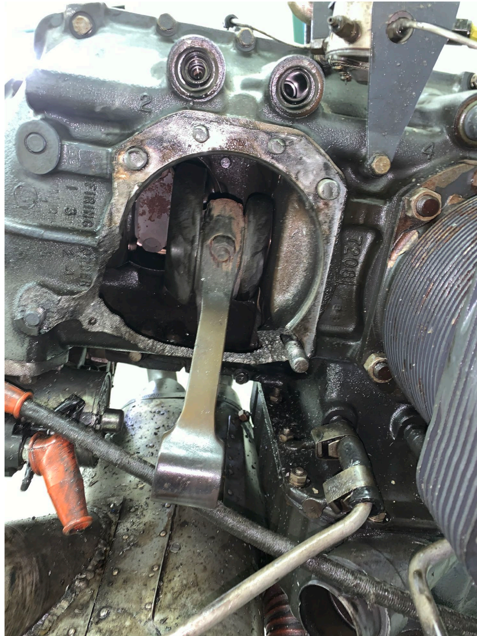
Photo 4 - NTSB Digital Photograph. View Showing the No. 2 Cylinder Pad of the Crankcase. Note the heat Discoloration of the Connecting Rod Consistent with Lack of Lubrication.
