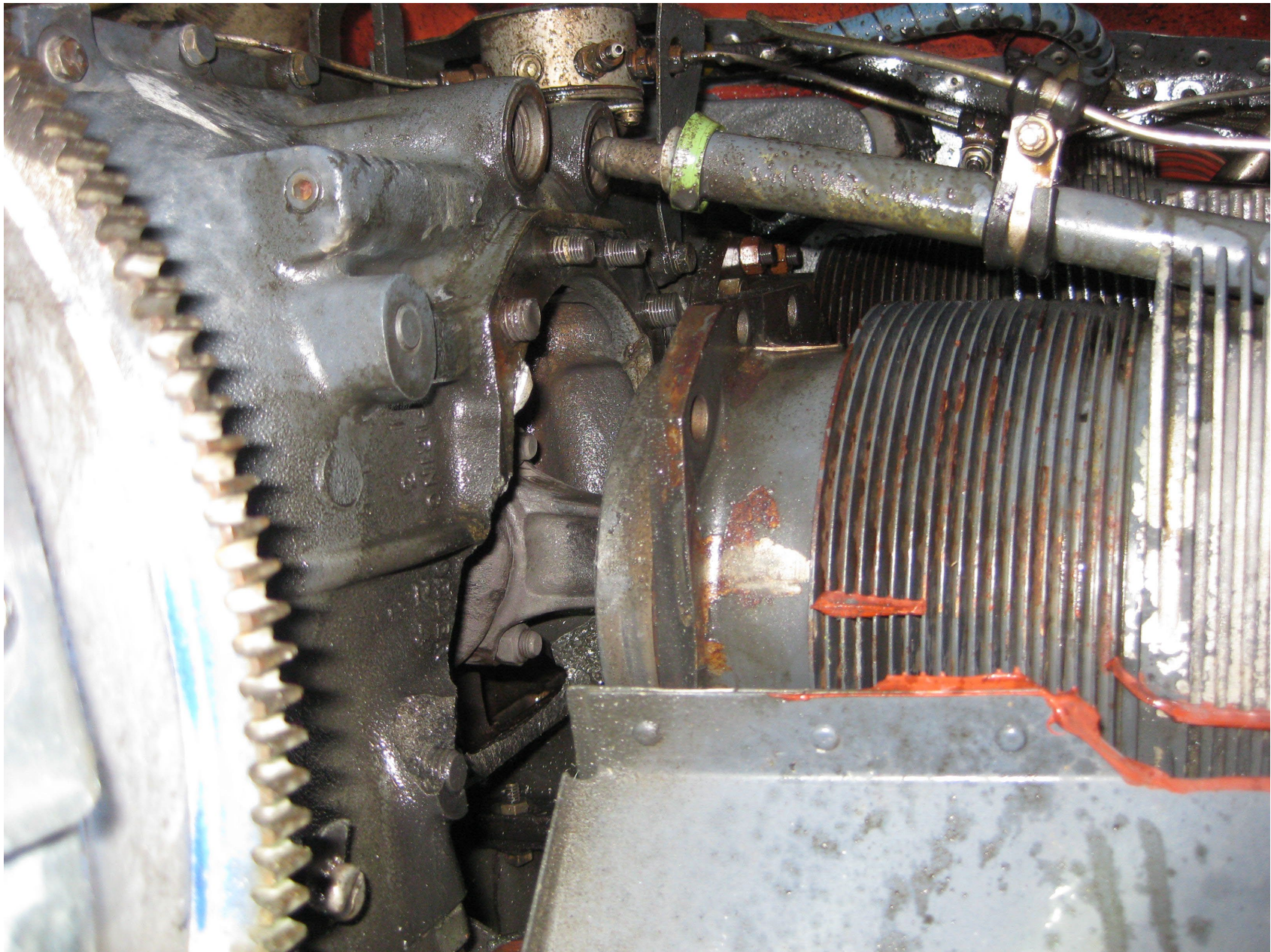
Photo 3 - Digital Photograph Provided by FAA. View Showing Separated No. 2 Cylinder From the Crankcase.
