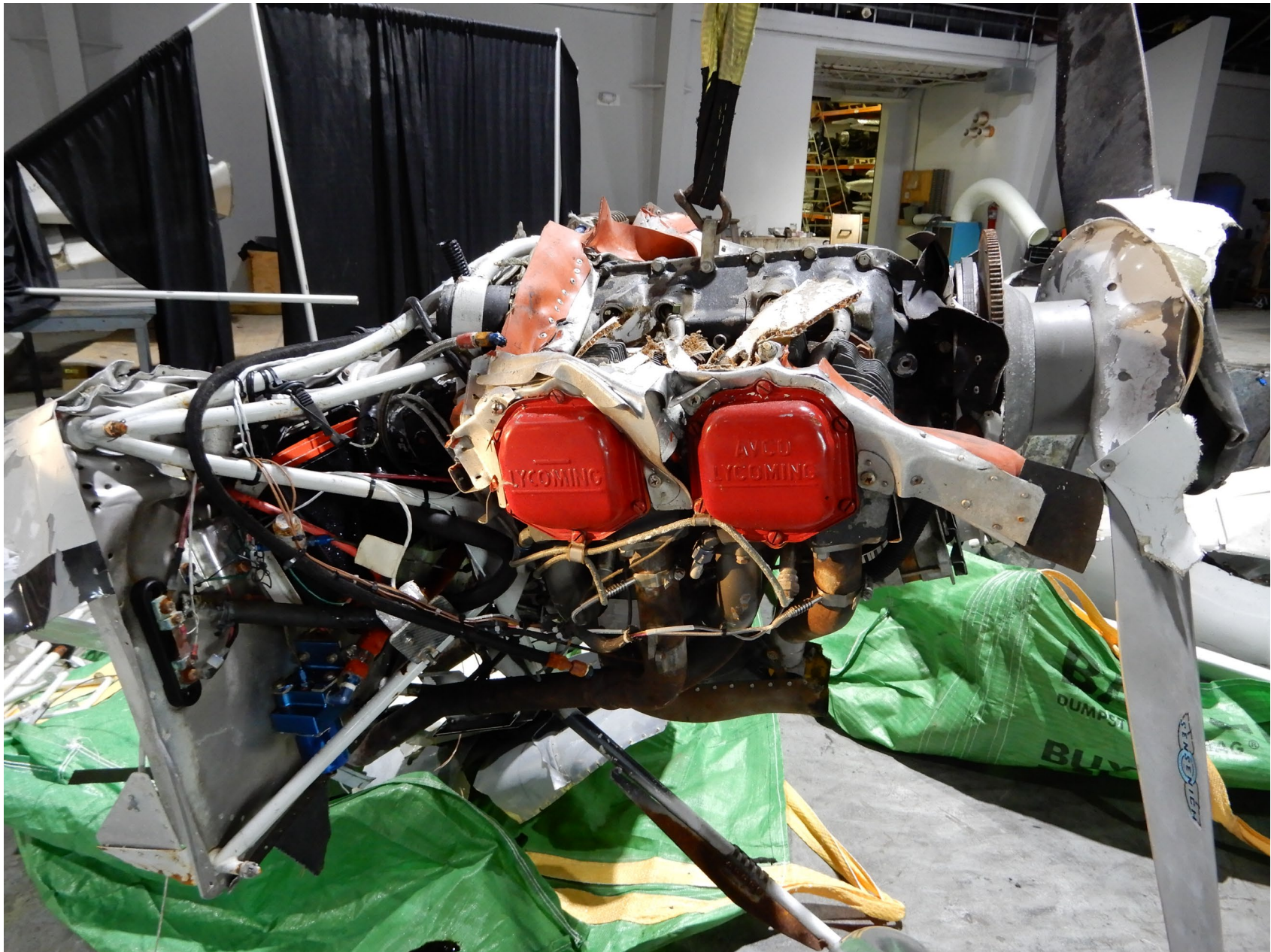
Photo 3 – Engine and Propeller (NTSB Photo)
