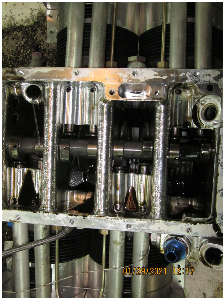
Photo 19 – Camshaft and Lifters – Courtesy of UL Power
