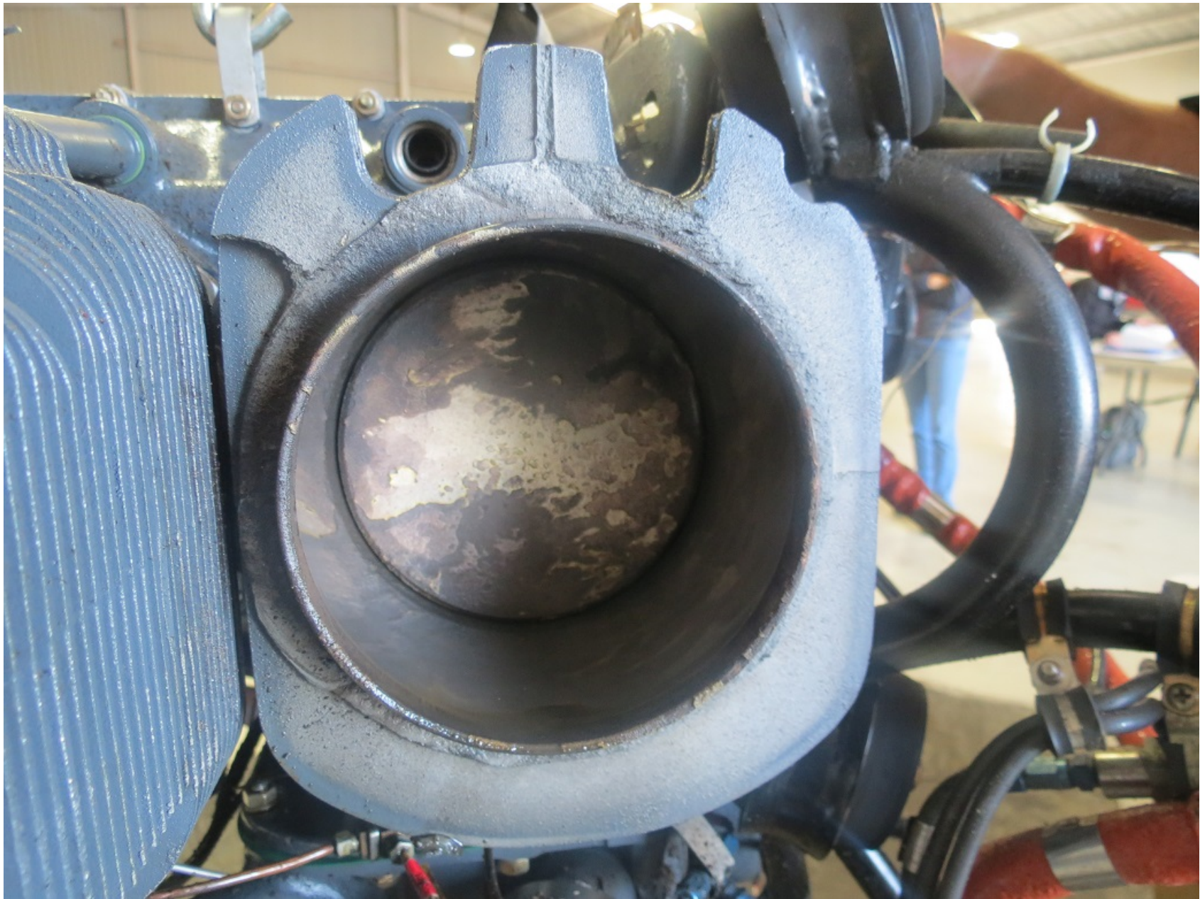
Photo 4 – Number Four Cylinder (Photo Courtesy of Lycoming)
