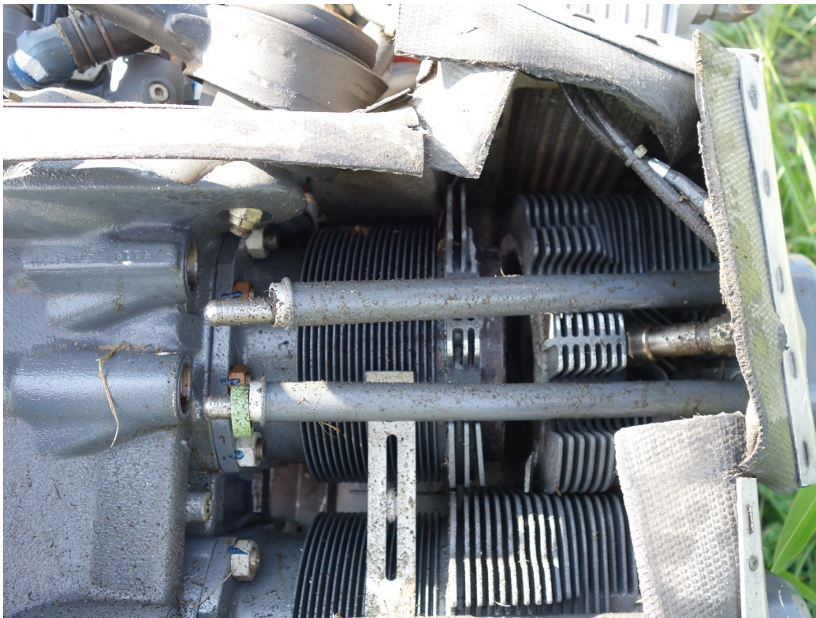
Photo 3 – Left Side of Engine (Photo Courtesy of Piper)
