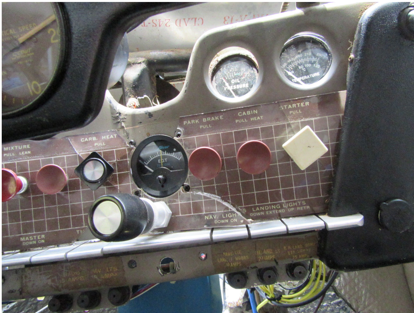
Photo 8 – Mixture Control, Carburetor Heat Control, and Throttle Control – Courtesy of FAA
