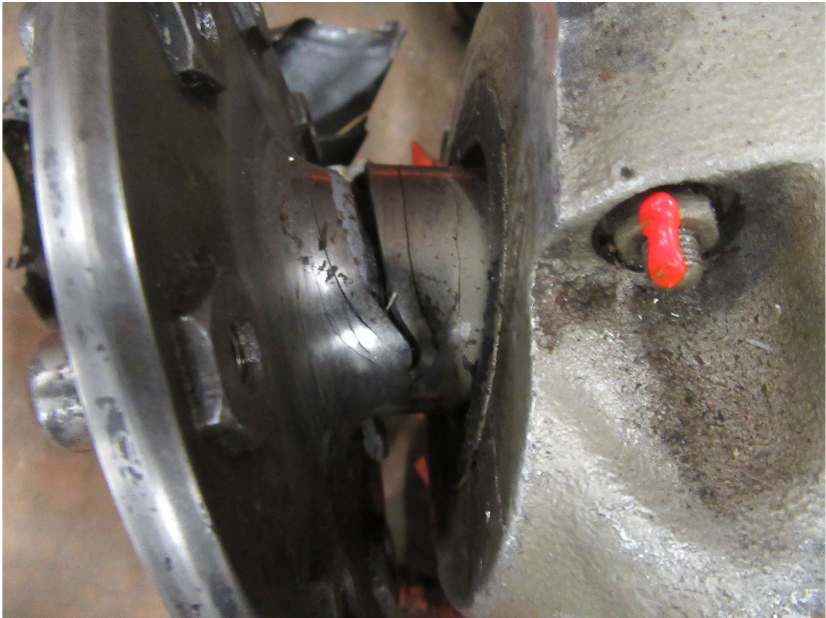
Photo 11 -Side View of Crankshaft Fracture – Courtesy of FAA
