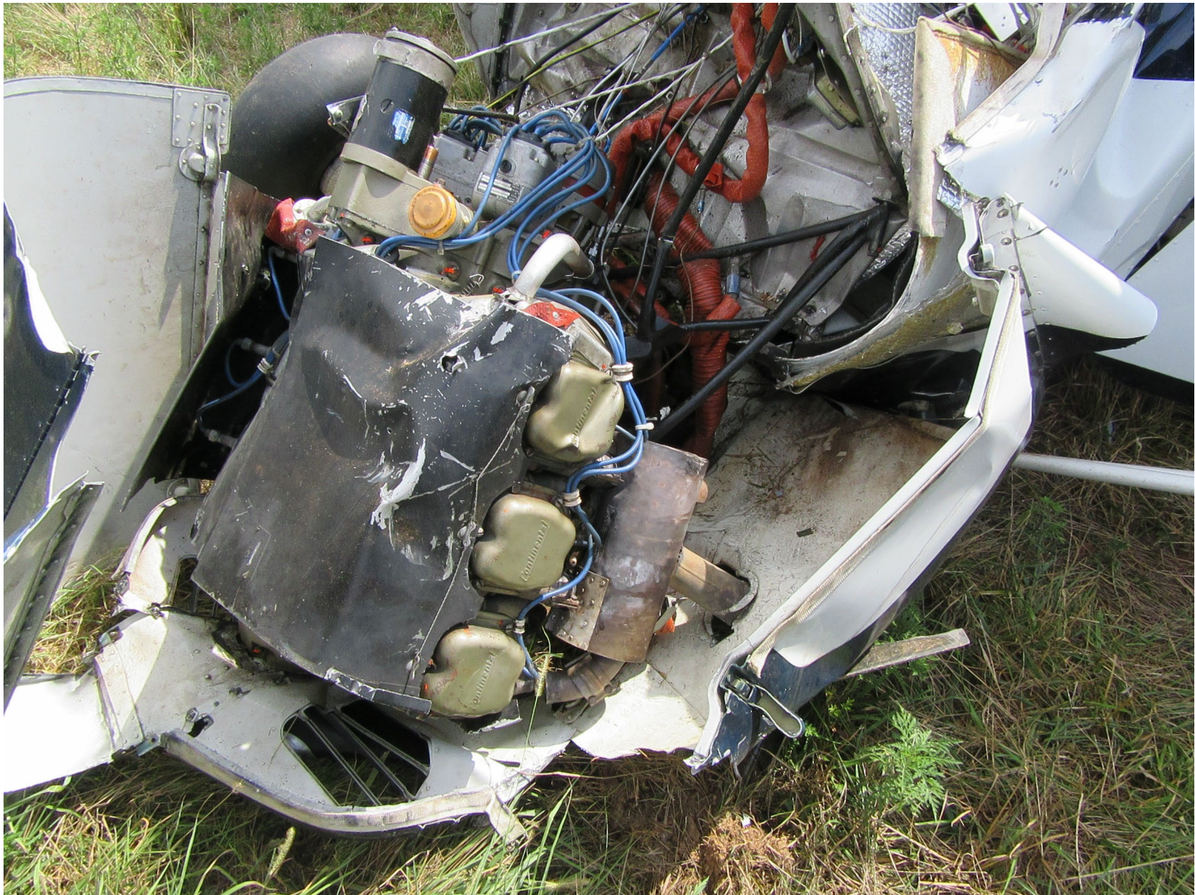
Photo 6 – Engine – Courtesy of FAA
