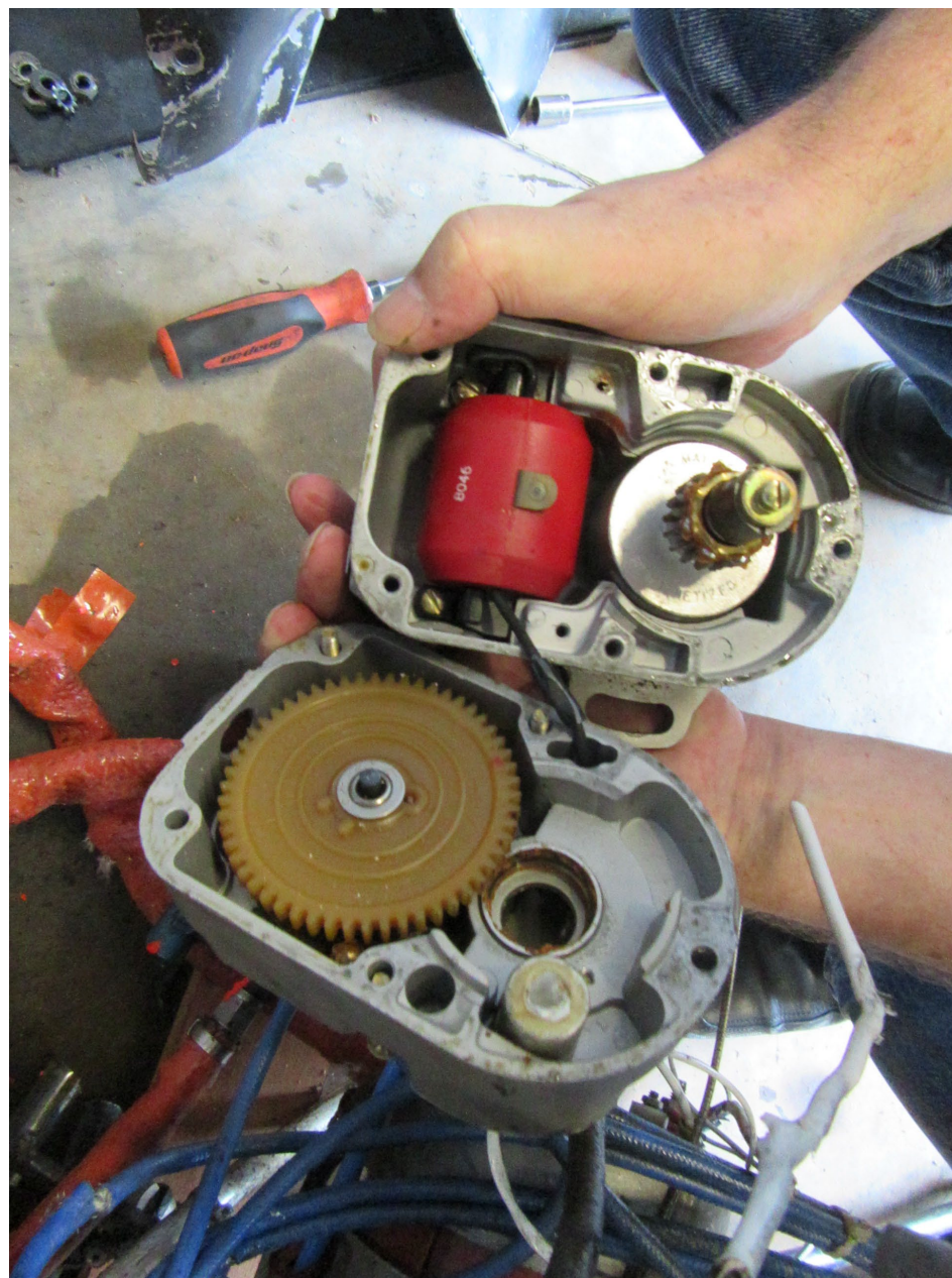
Photo 14 – Inside of Right Magneto – Courtesy of FAA
