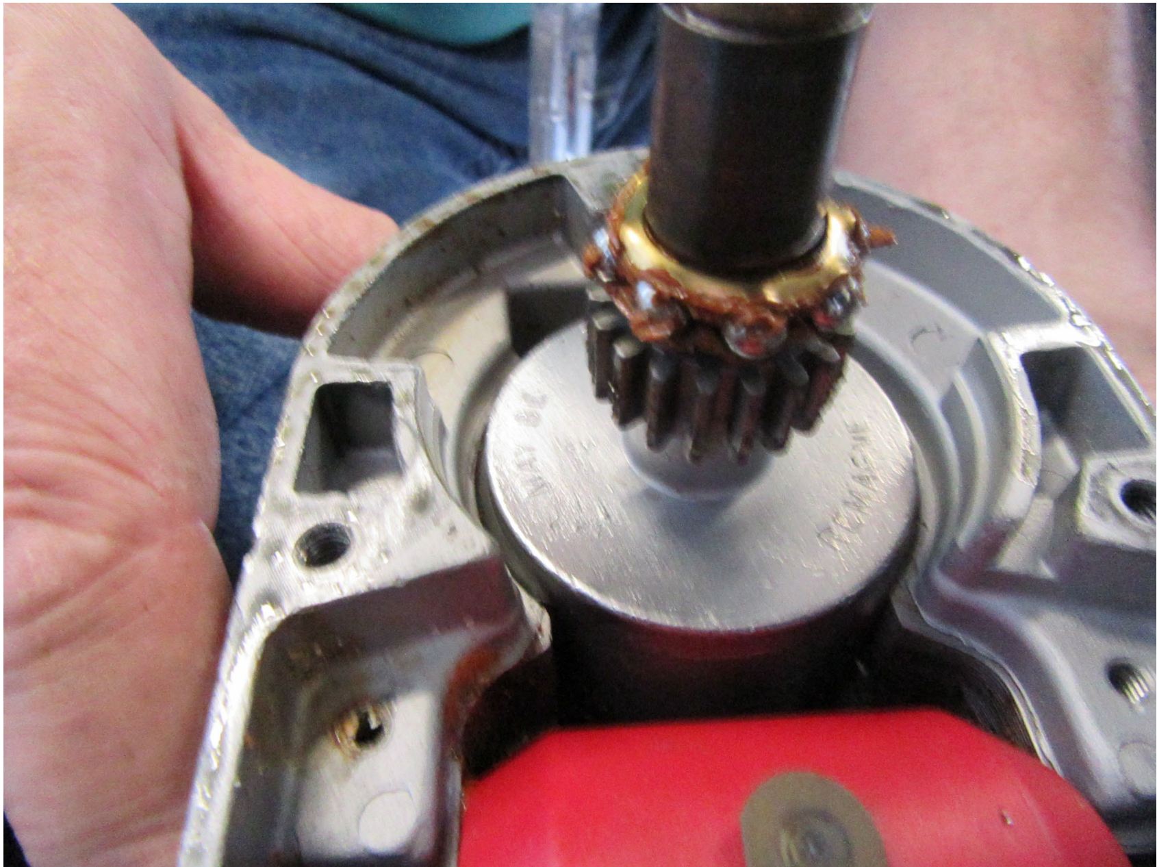
Photo 15 – Impact Damaged Bearing – Courtesy of FAA
