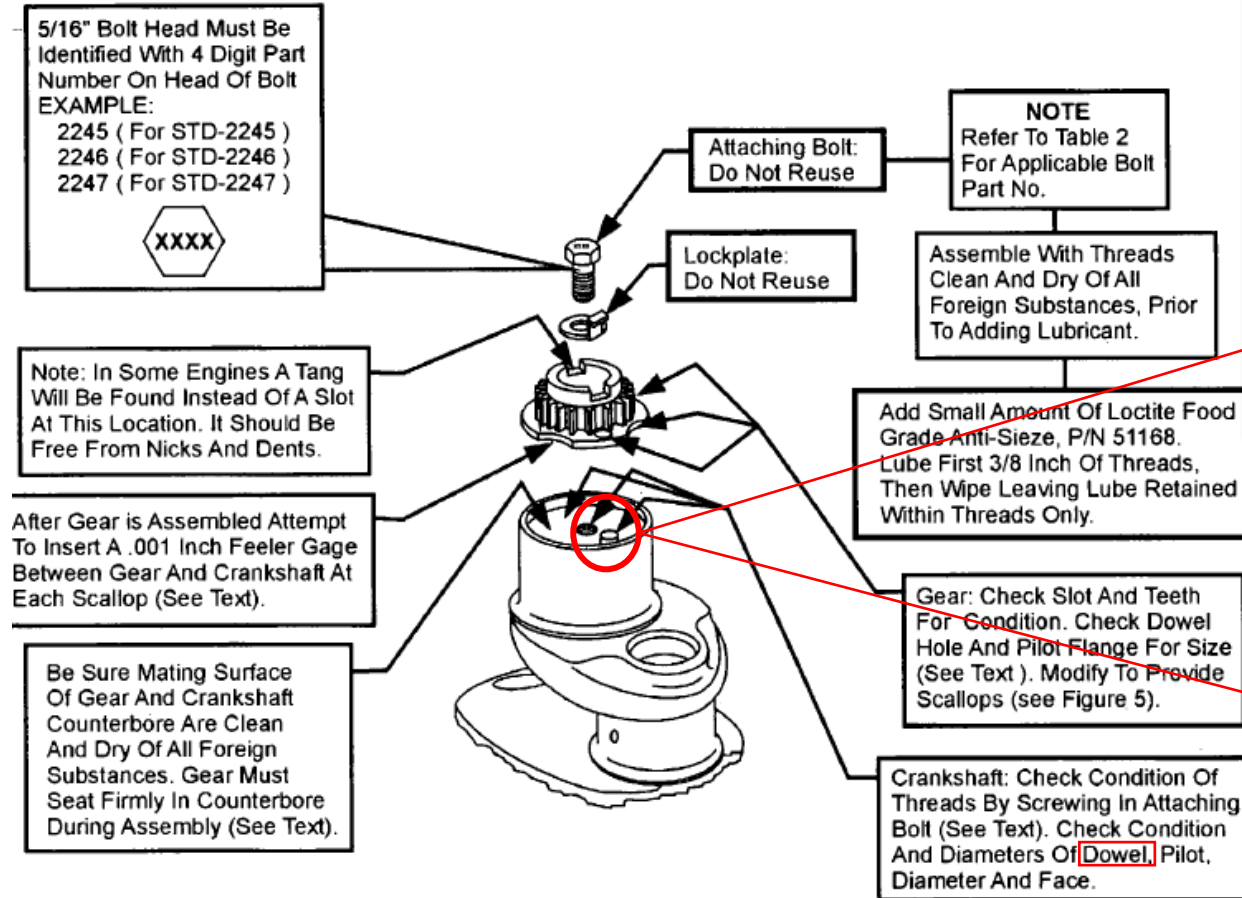
Figure 6. Rear End View of Crankshaft Showing Associated Parts
