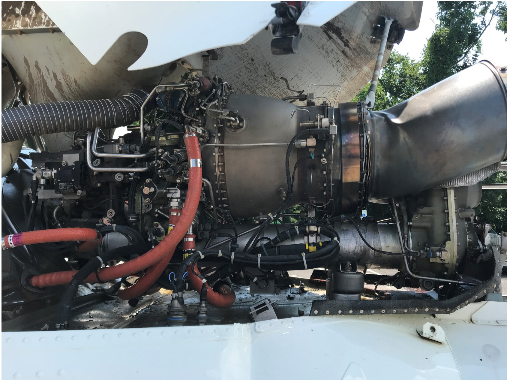
Photo 7 – View of Engine (Photo Courtesy of Safran Helicopter Engines)
