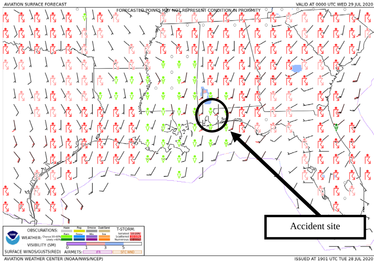
Figure 1 – GFA Surface Forecast valid at 1900 CDT with forecast issued at 1401 CDT
