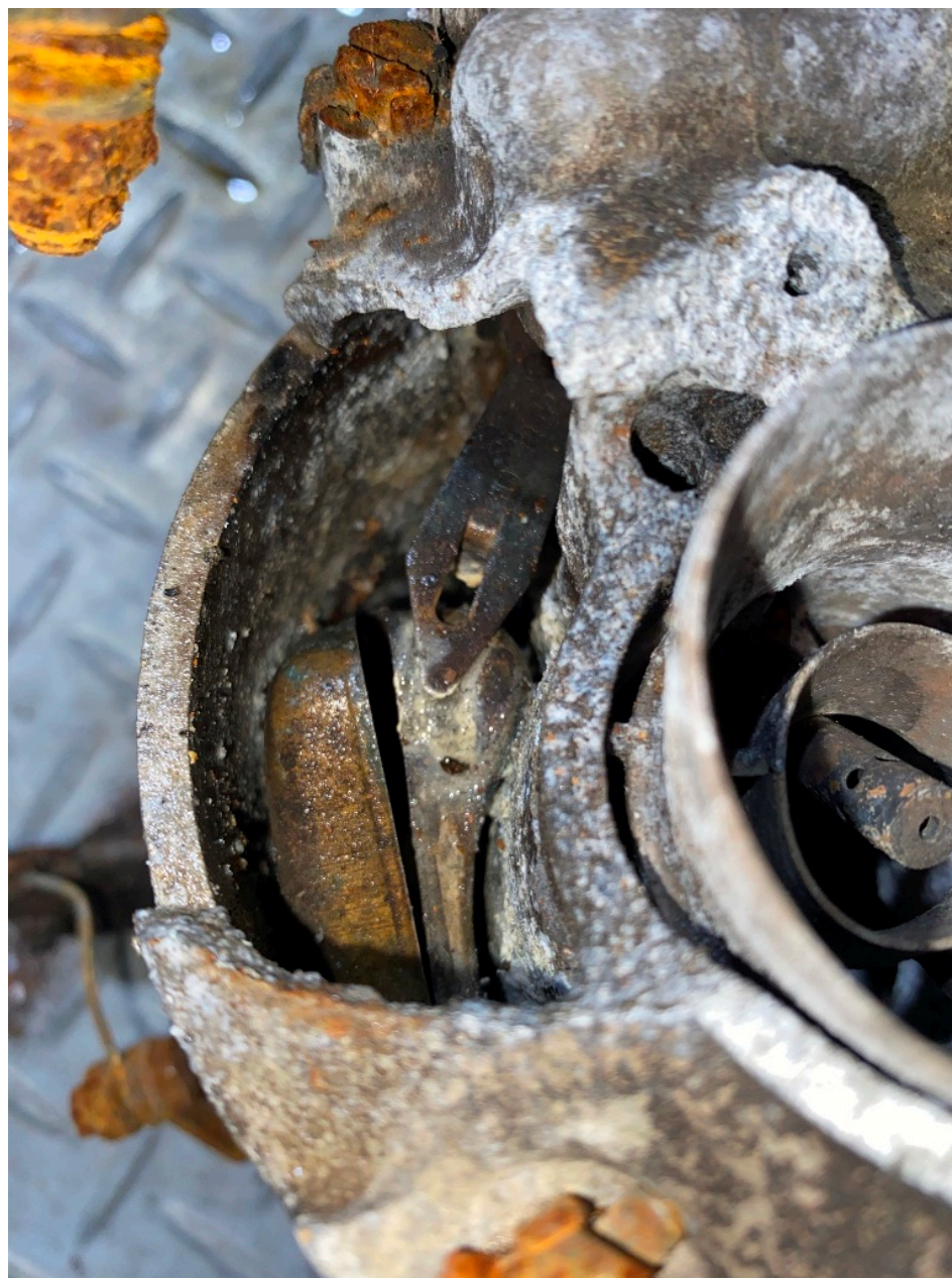
Photo 6 - Digital Photograph From Florida Air Recovery. View Showing the Carburetor Bowl and the Split Halves of the Brass Float.
