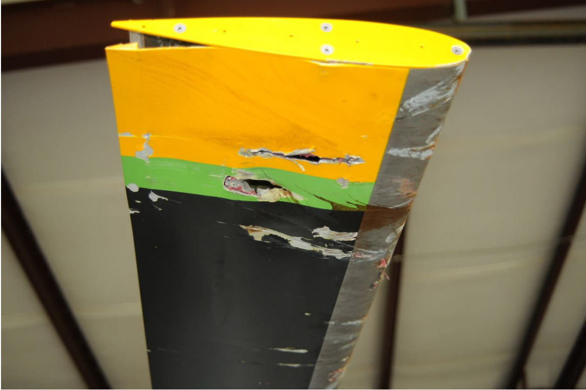
Photograph 6 – Accident helicopter – Post accident examination of rotor blades.
