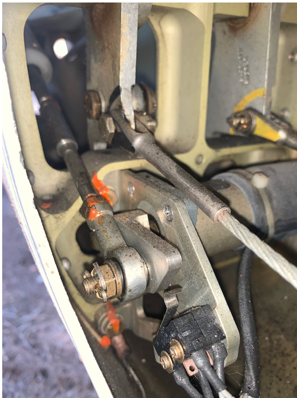
Photo 4 - Digital Photograph From Atlanta Air Salvage. View of the Position of the Pitch Trim Actuator which was near Full Airplane Nose Down.
