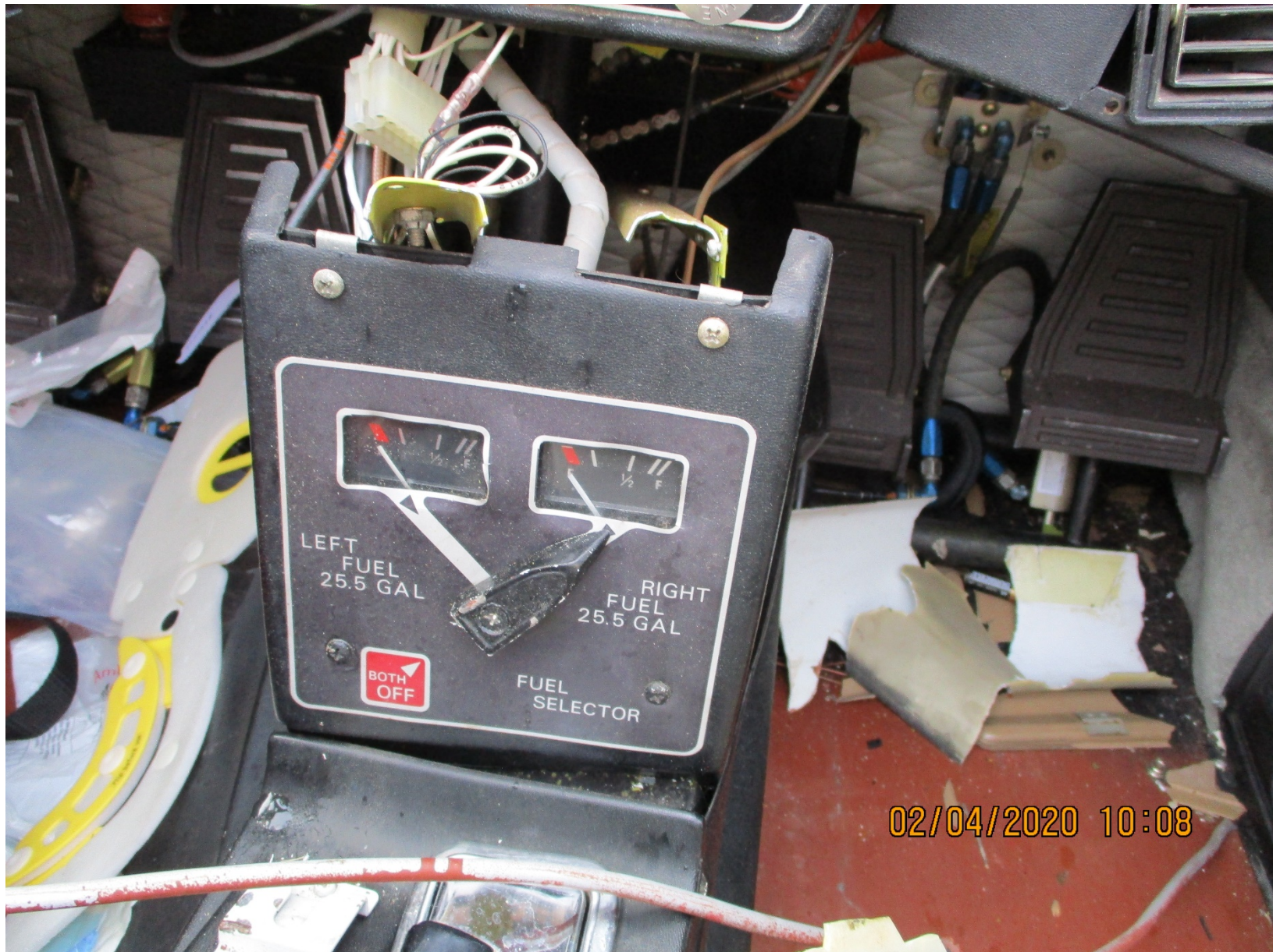
Photo 3 – Fuel Selector
