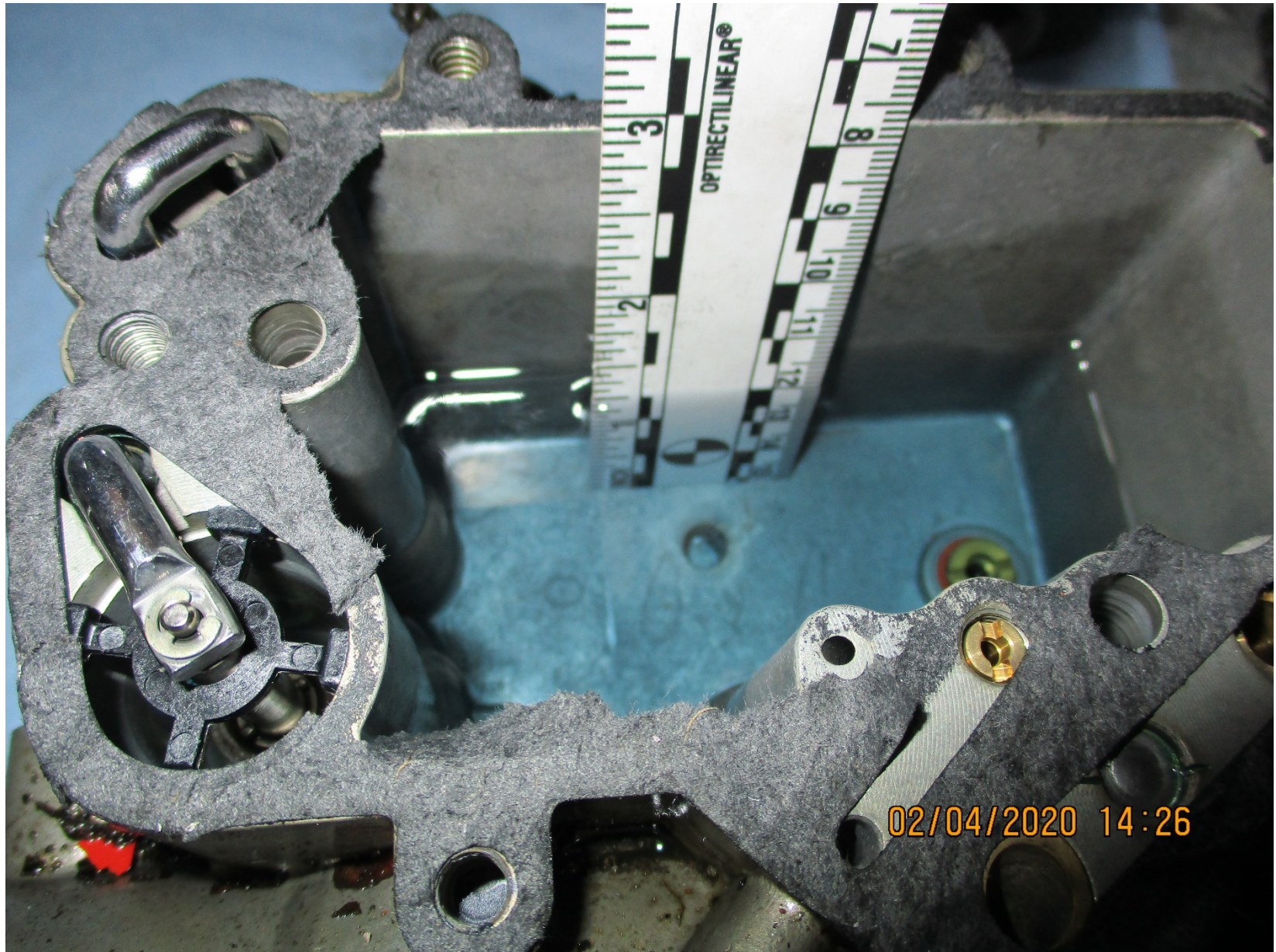
Photo 4 – Fuel in carburetor
