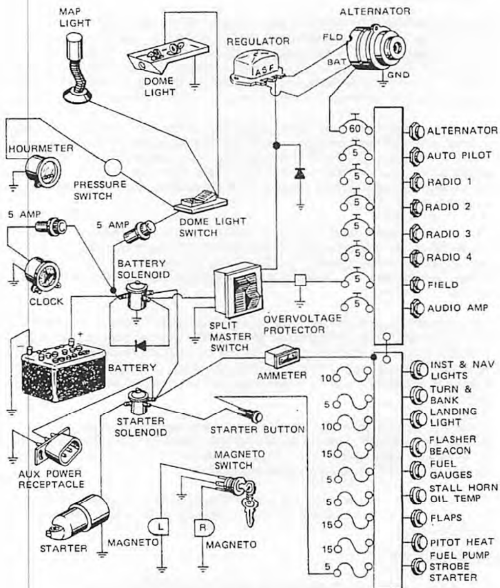
Figure 7-3, Electrical System
