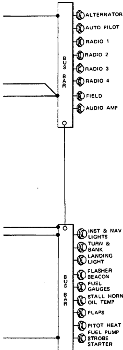
Figure 7-3 Electrical System (Sheet 2 of 2)
