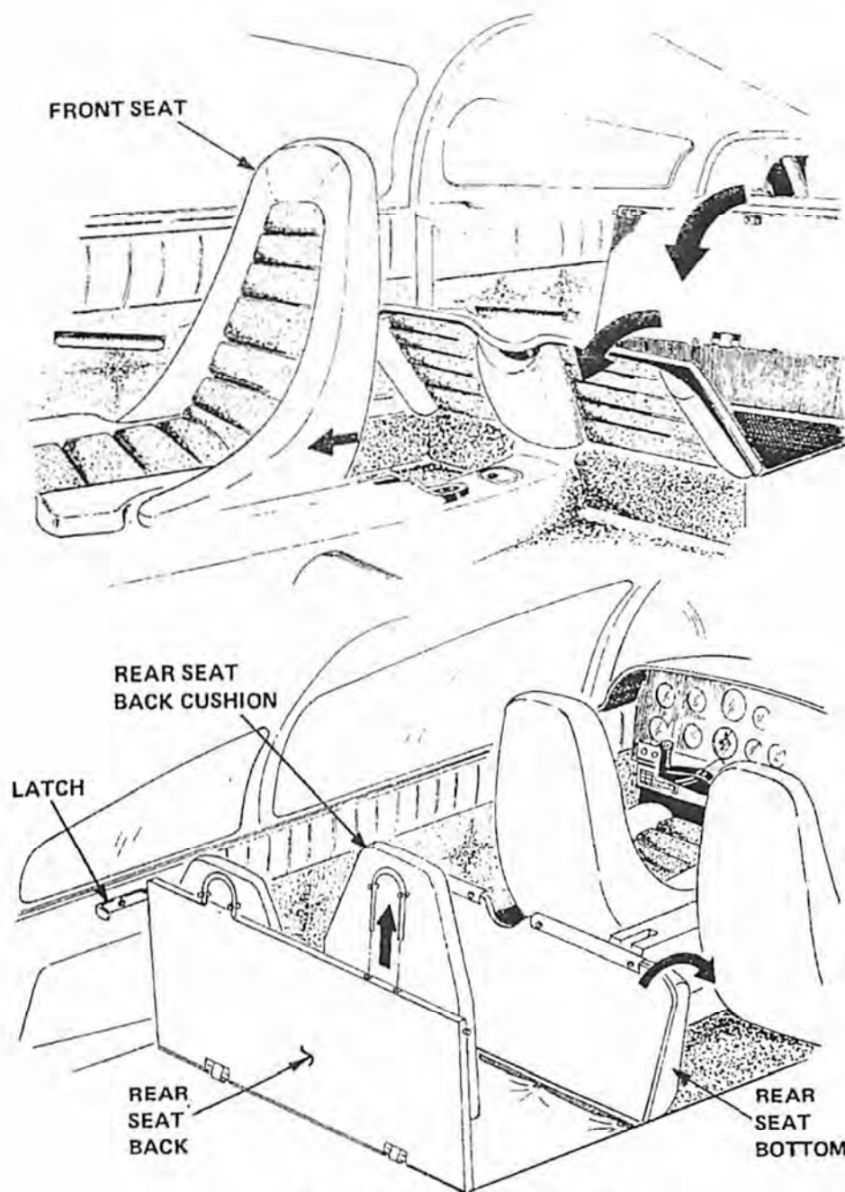
Figure 6-6. Rear Seat Stowage
