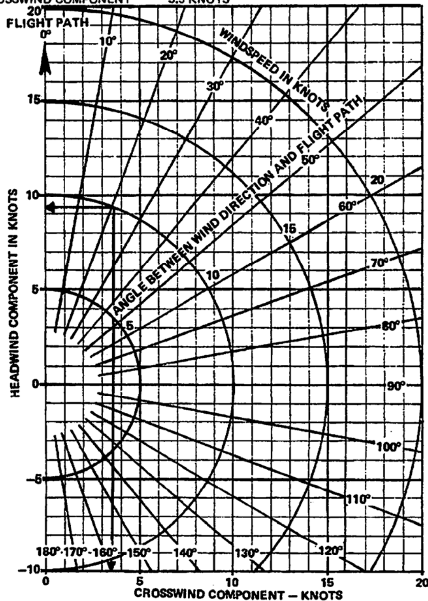
Figure 5-6. Crosswind Component Chart
