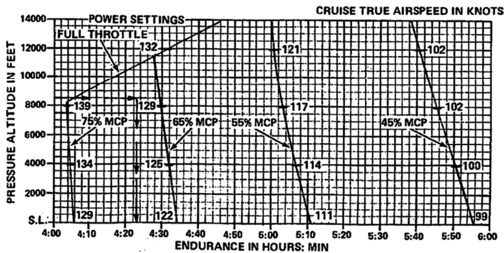
Figure 5-15. Endurance Profile - 51 Gallons Fuel
