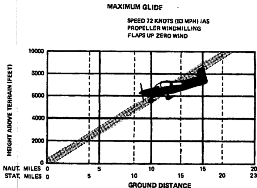
Figure 3.1 Maximum Glide
