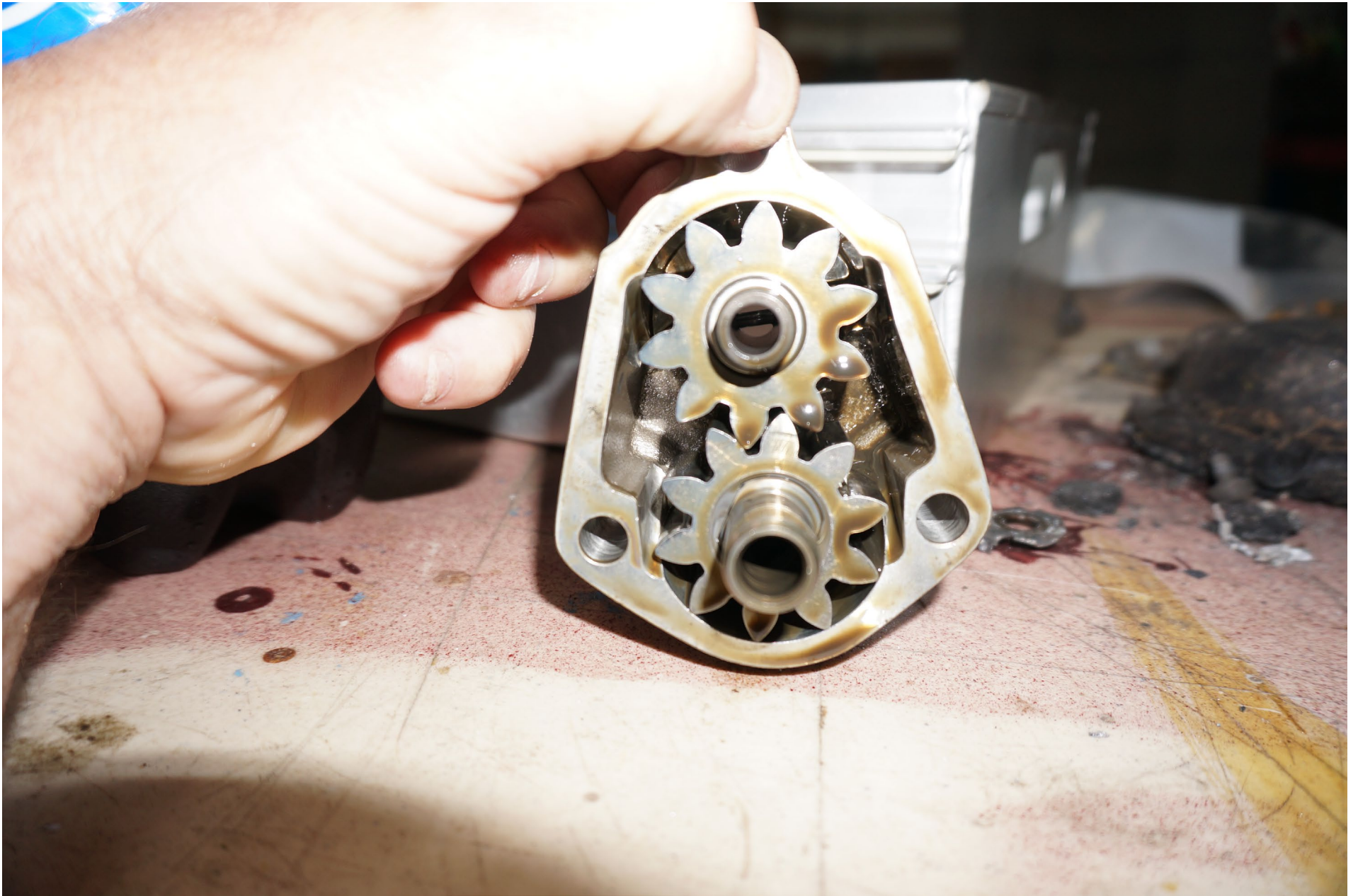
Photo 18 – Interior of Oil Pump
