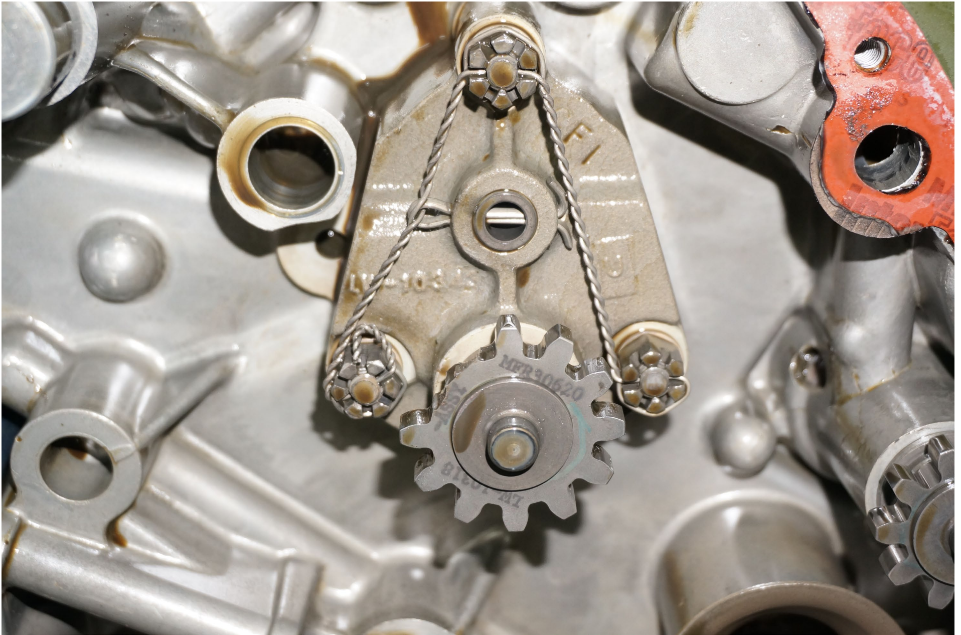
Photo 17 – Oil Pump Drive Gear
