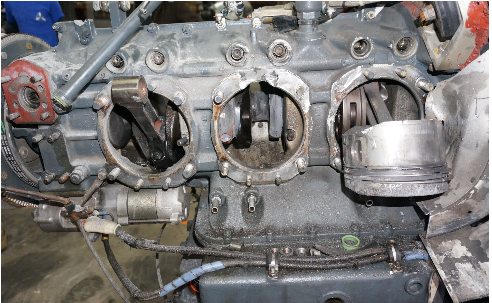
Photo 14 – Left Side View of Engine After Cylinder Removal
