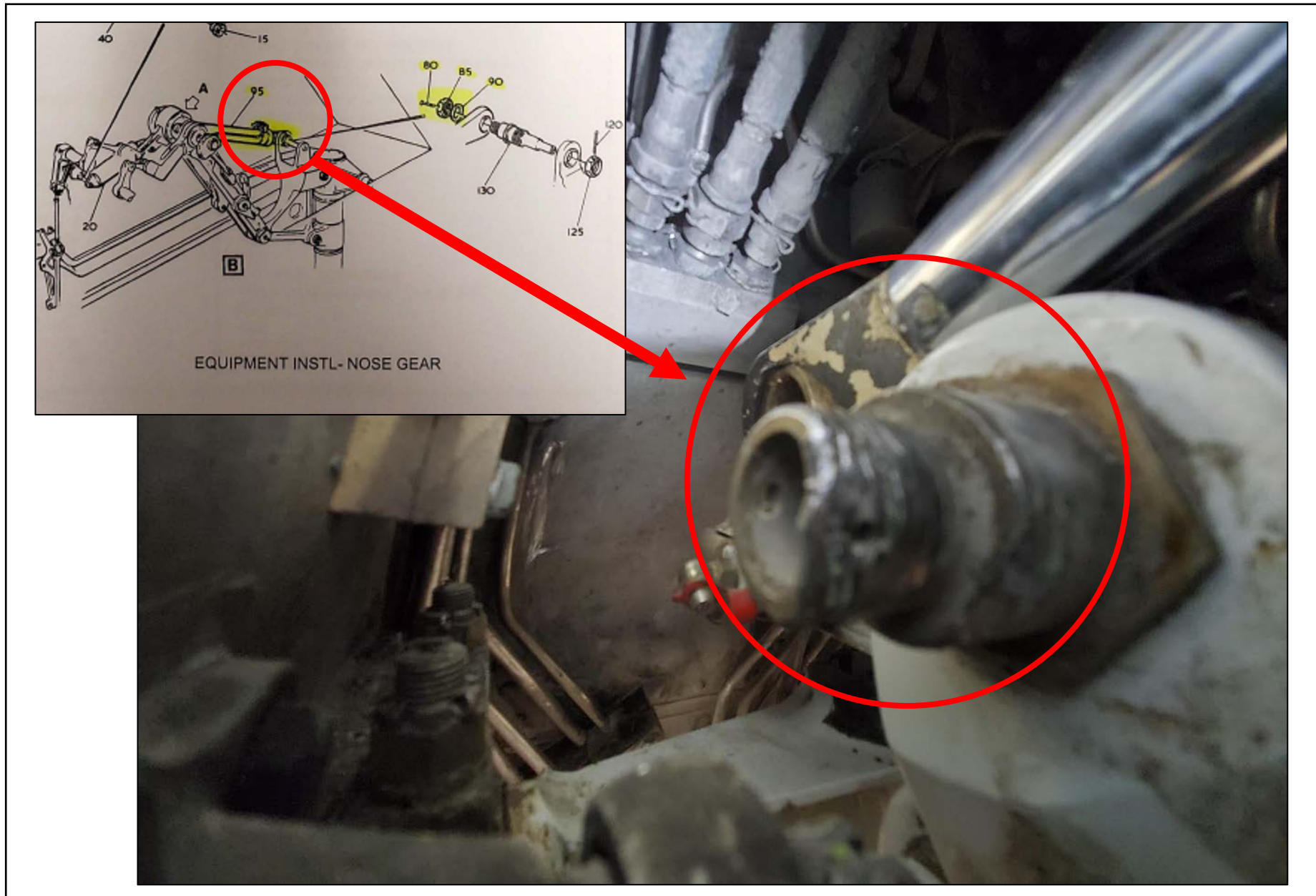
Photo 1 – View of the nose landing gear actuator (Photograph Courtesy of FAA)
