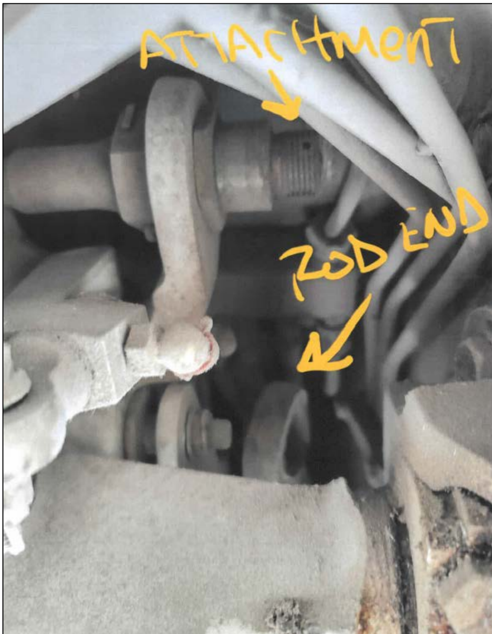
Photo 1: View of actuator and its attach point (Photo Courtesy of Delta Private Jets)
