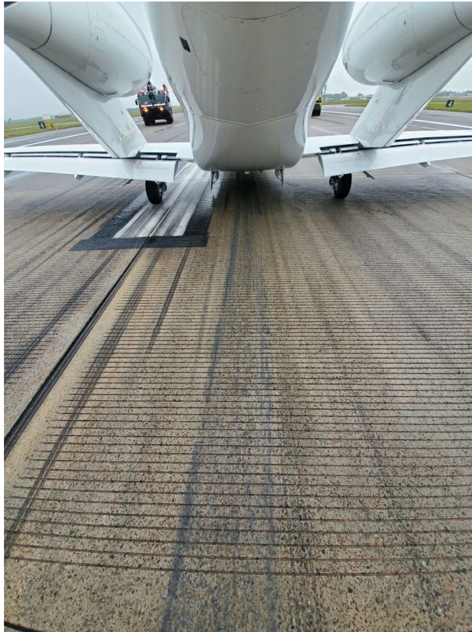
Photo 3 – View of aft of airplane
