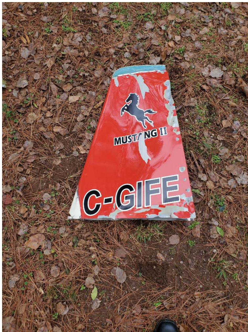
Photo 2 – Vertical Stabilizer (Photo Courtesy of FAA)
