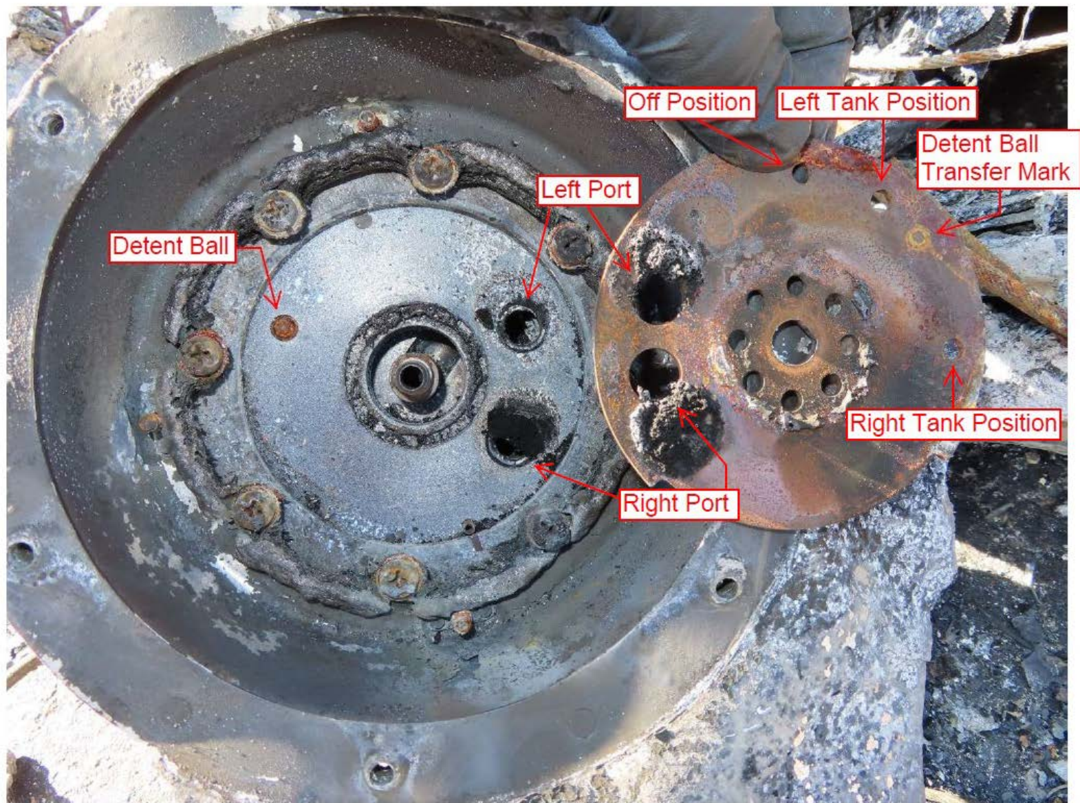
Photo 7 – View of Fuel Selector Plate Witness Marks (Piper)
