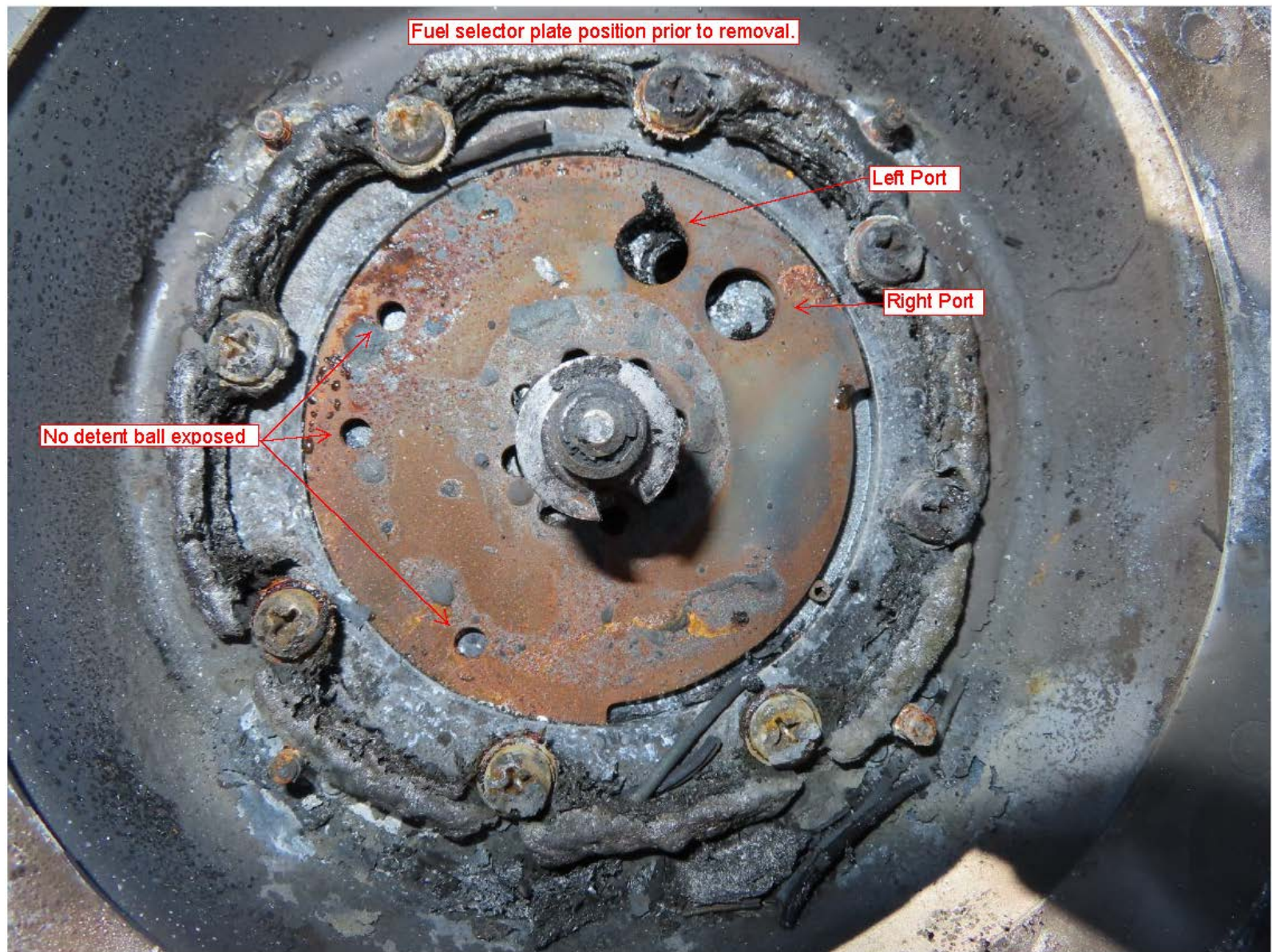
Photo 6 – View of Fuel Selector Plate as Found (Piper)
