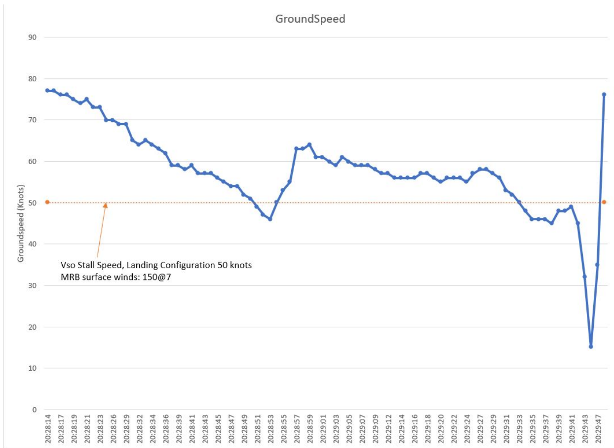
Figure 3 Groundspeed (last 90 seconds)
