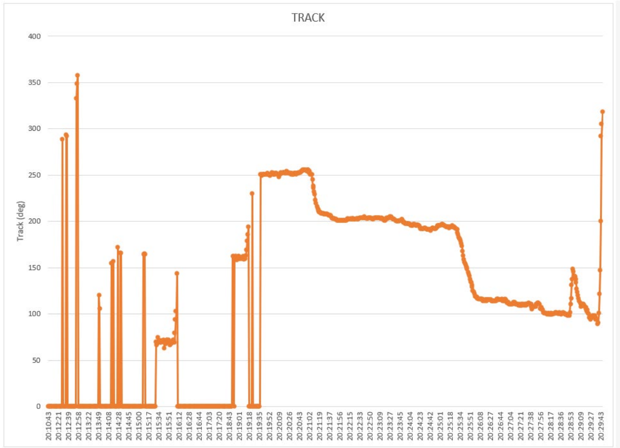
Figure 8 - Ground Track (entire flight)
