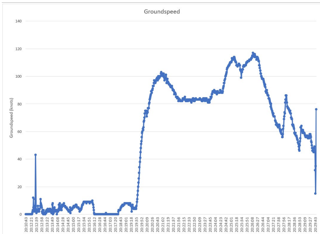
Figure 6 - Groundspeed (entire flight)
