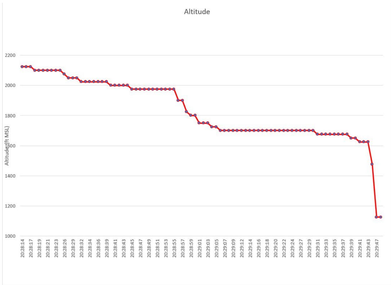
Figure 4 – Altitude (last 90 Seconds)
