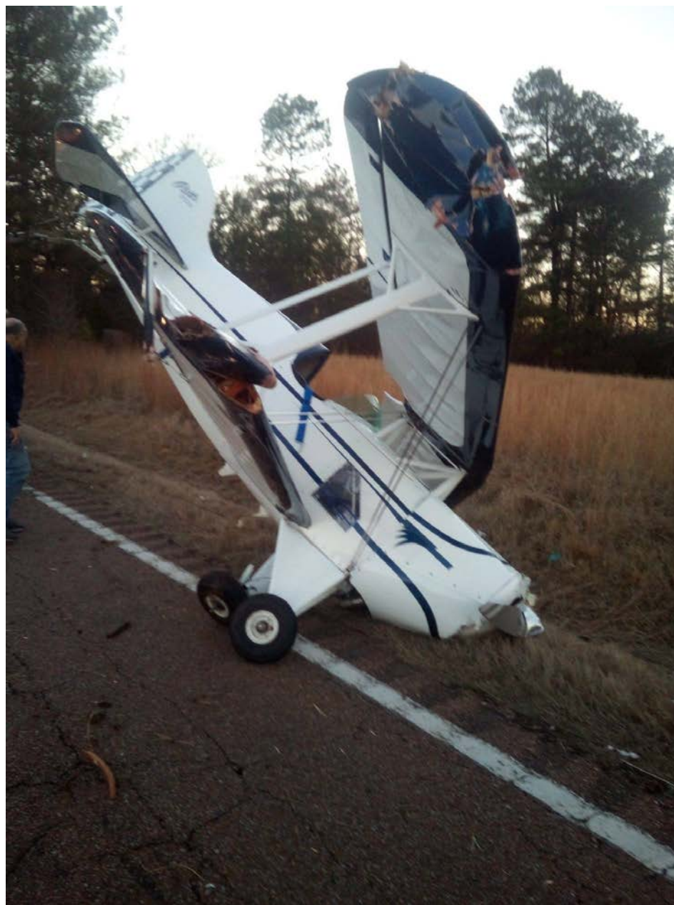
Photo 1 – View of the right side of the wreckage and damage to right wing. (Photo courtesy of the pilot)
