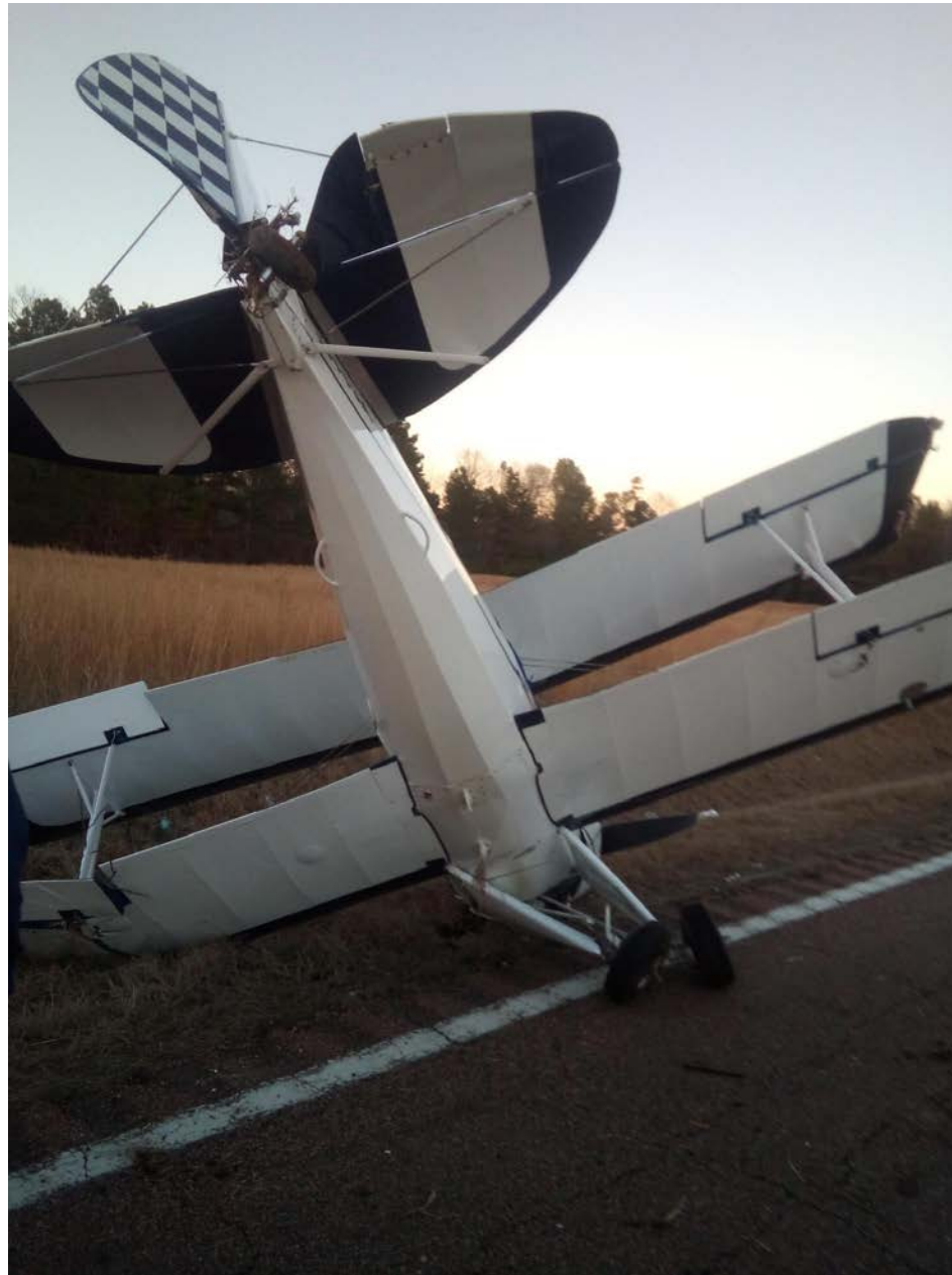
Photo 2 – View of the belly of the airplane, broken main landing gear, and damage to left wing. (Photo courtesy of the pilot)
