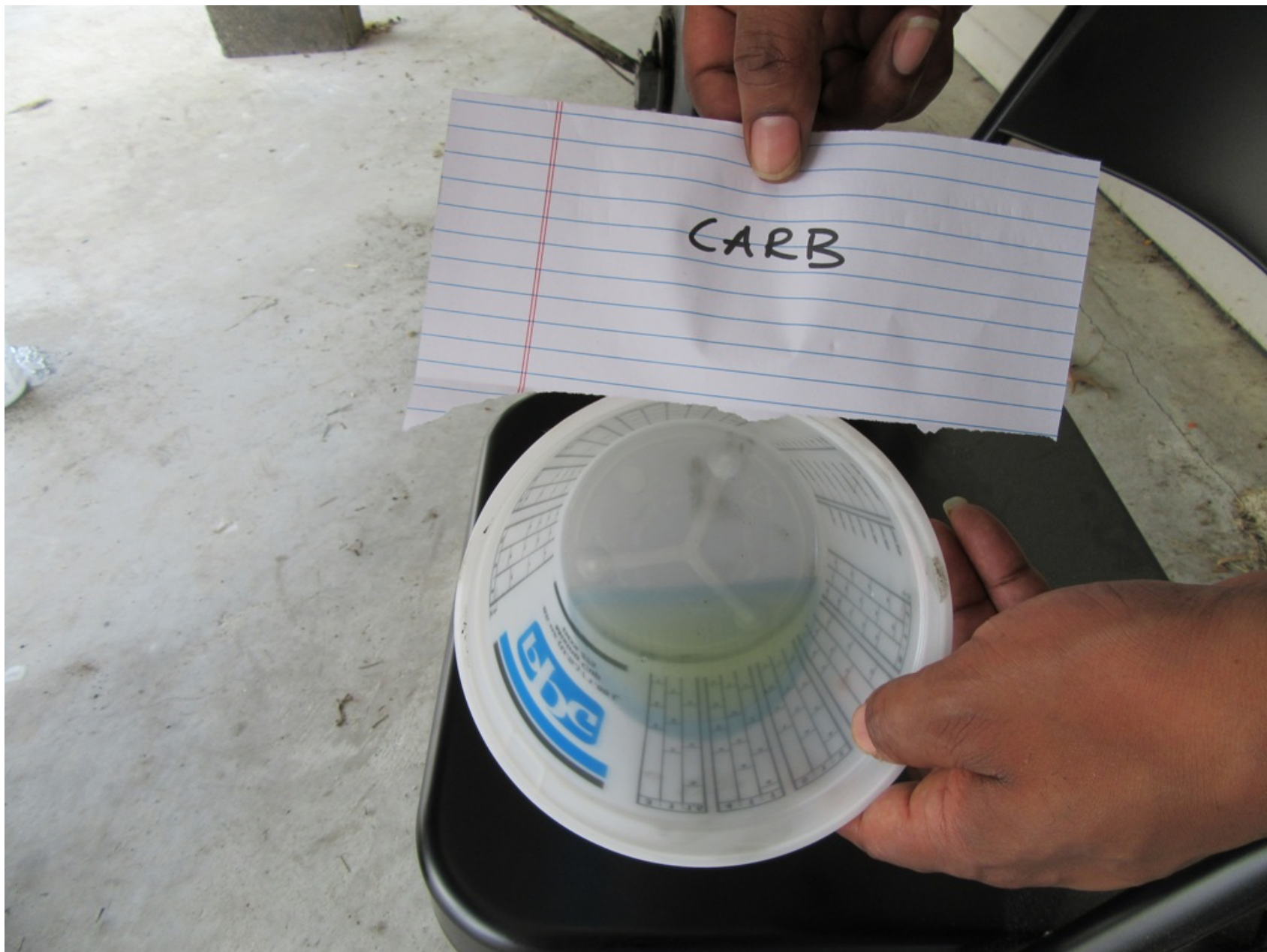
Photo 2 – Fuel Sample From Carburetor (Photo Courtesy of FAA)
