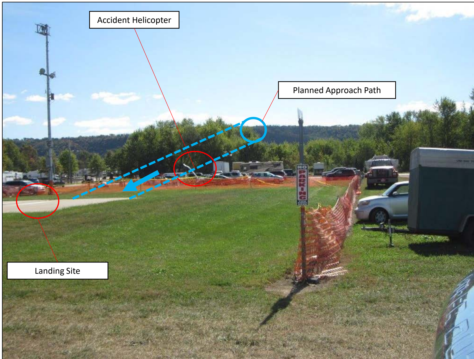
Figure 2 – View of the accident helicopter, the landing site, and planned approach path
