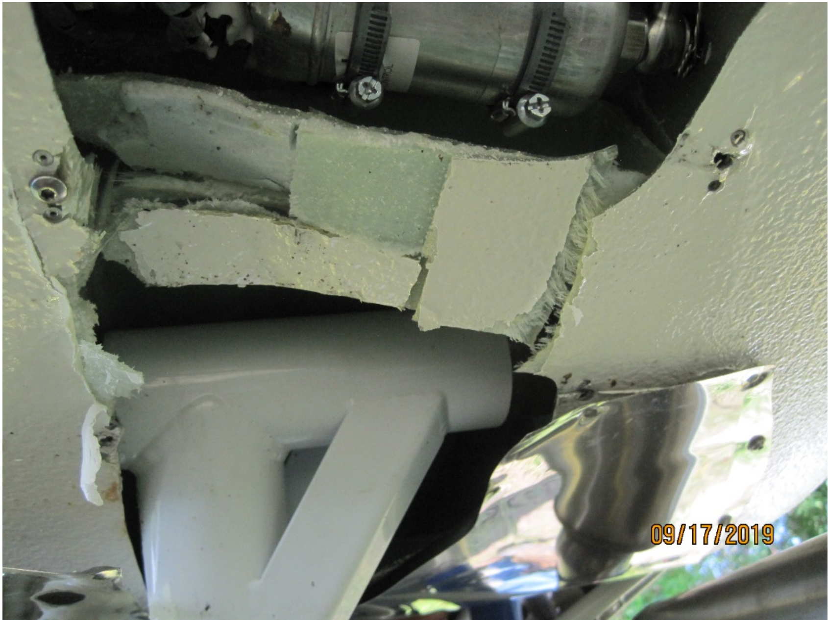
Photo 4 - Fuselage structure aft of the nose landing gear. (Photo Courtesy of FAA)
