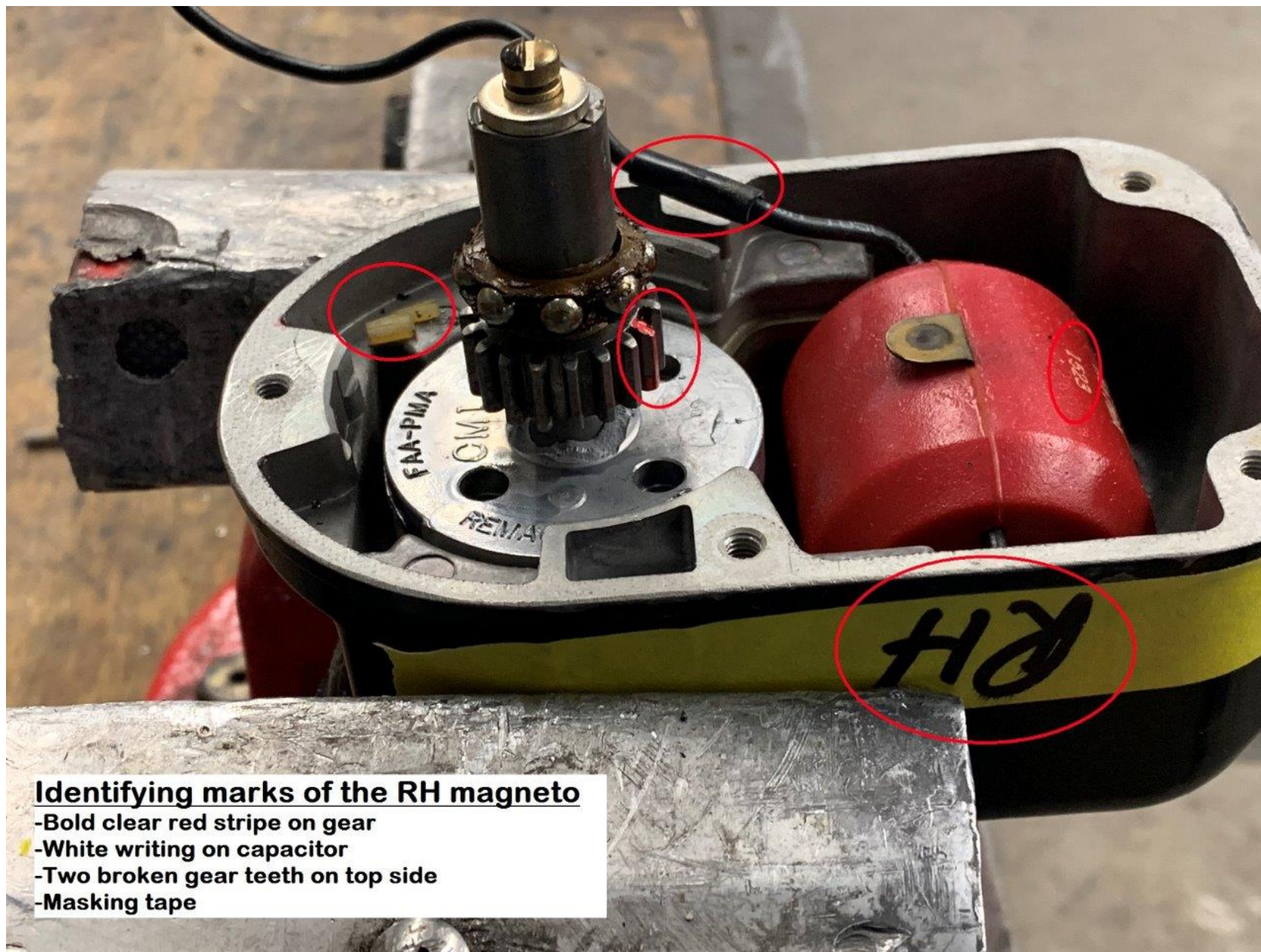
Photo 4 – View of Right Magneto During Disassembly (Myers Aviation)
