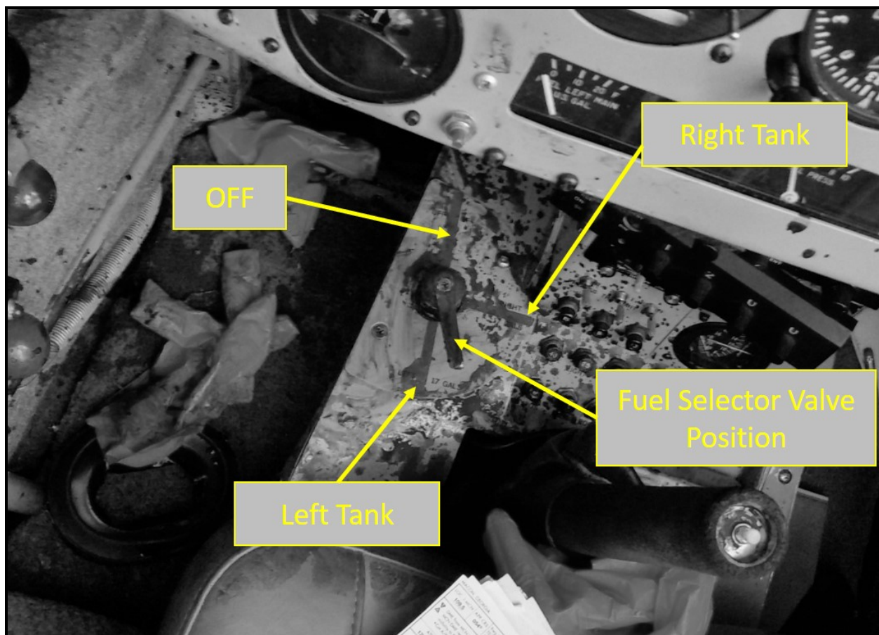
Photograph 2 2 – Accident airplanes fuel selector valve position.
