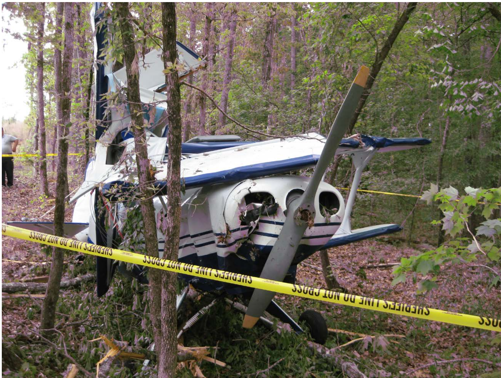
Photo 2 - View of Wreckage as Found Facing Opposite Direction of Travel (FAA)
