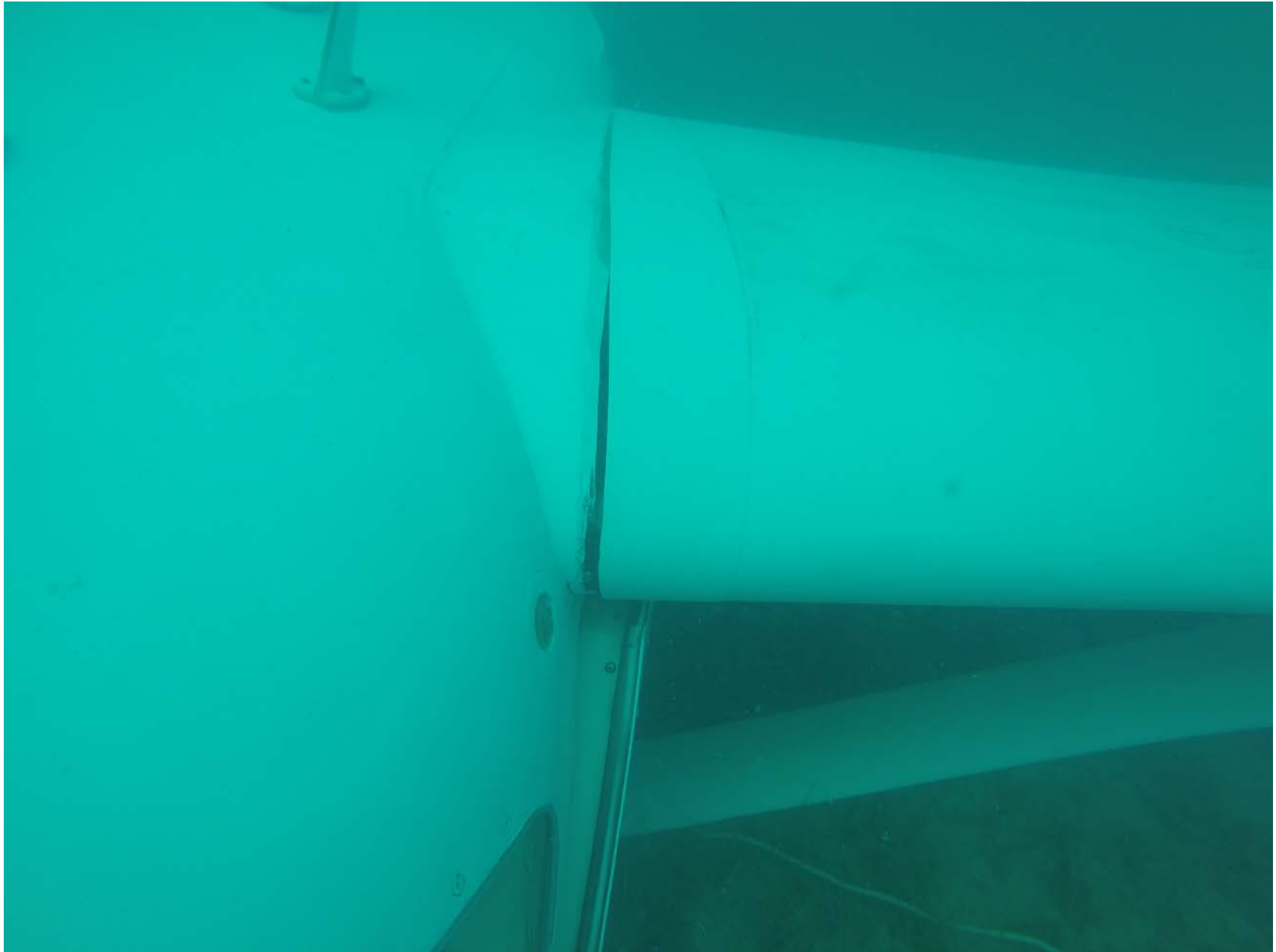
Photo 5 – Left Wing Root Damage (National Park Service Photo)
