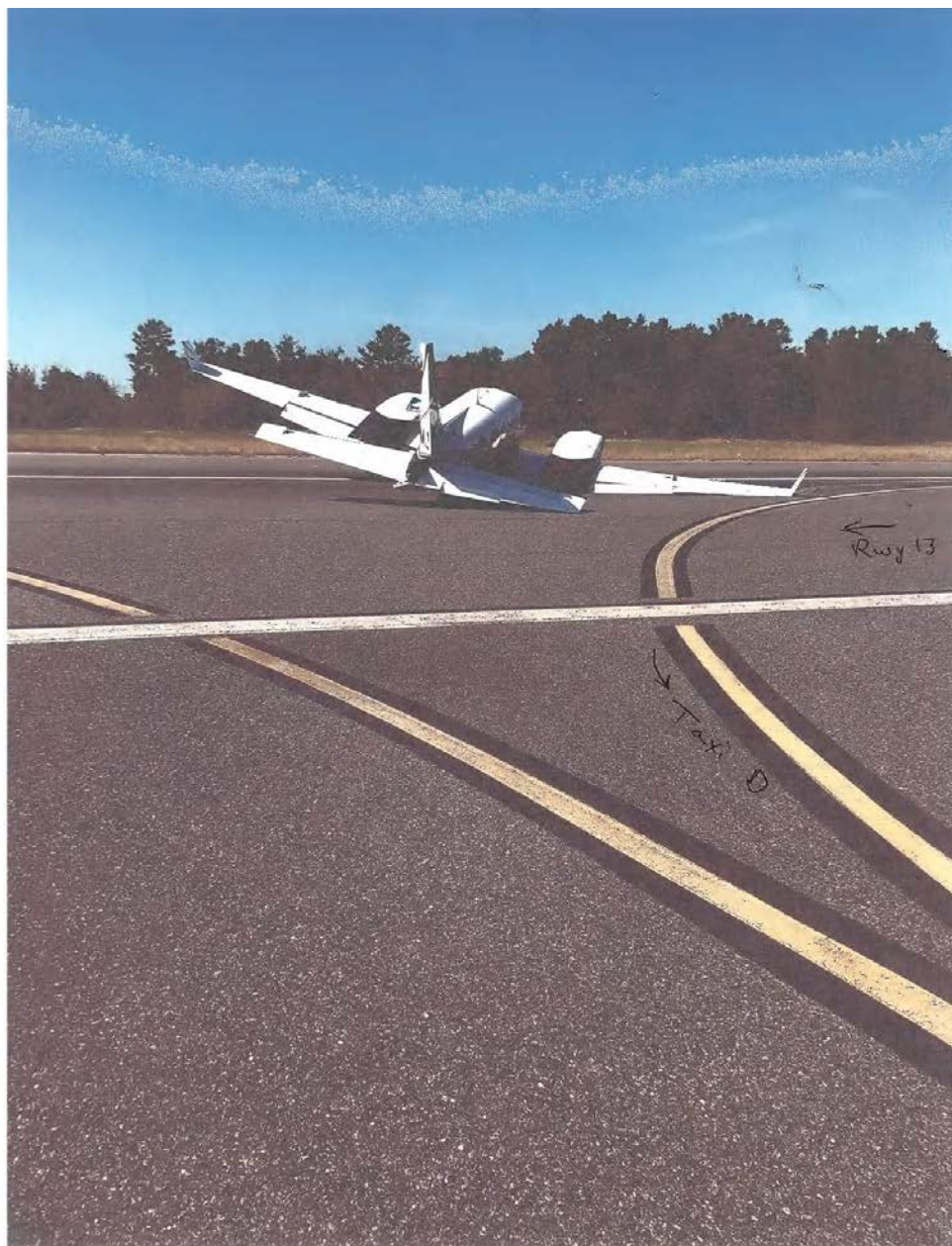
Photo 2 – View of airplane on taxiway with right gear collapsed
